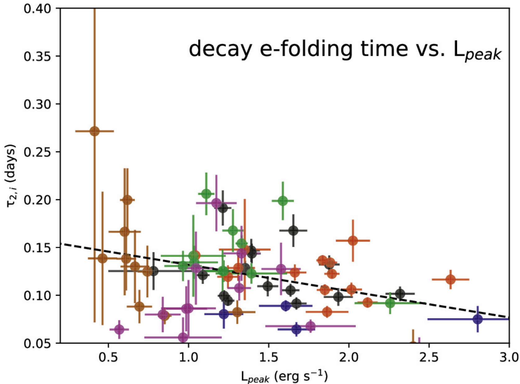
Figure C2. from Joheen Chakraborty et al 2024 Astrophys. J. 965 doi:10.3847/1538-4357/ad2941 https://dx.doi.org/10.3847/1538-4357/ad2941 © 2024. The Author(s). Published by the American Astronomical Society.
