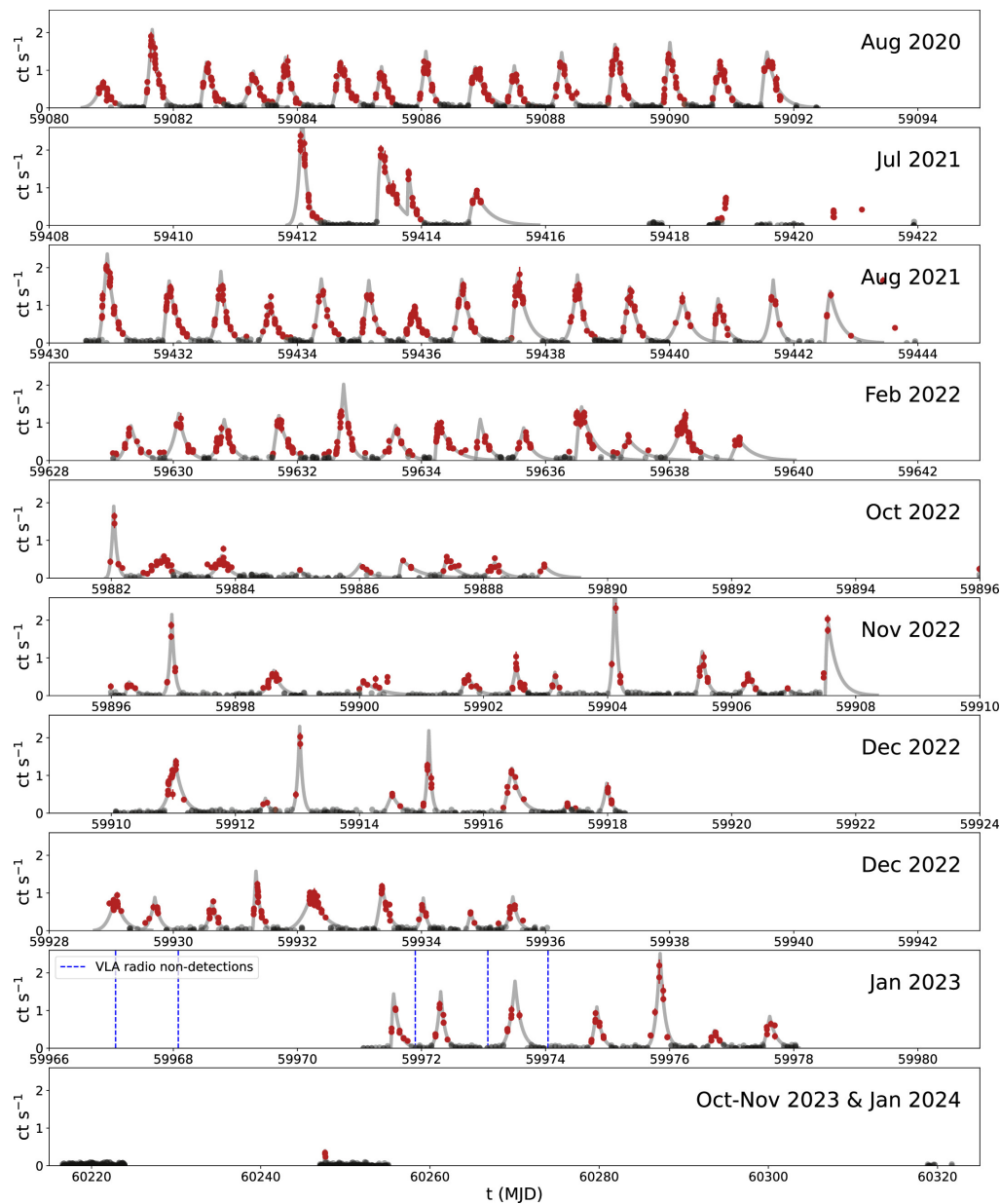
Figure 1. from Joheen Chakraborty et al 2024 Astrophys. J. 965 doi:10.3847/1538-4357/ad2941 https://dx.doi.org/10.3847/1538-4357/ad2941 © 2024. The Author(s). Published by the American Astronomical Society.
