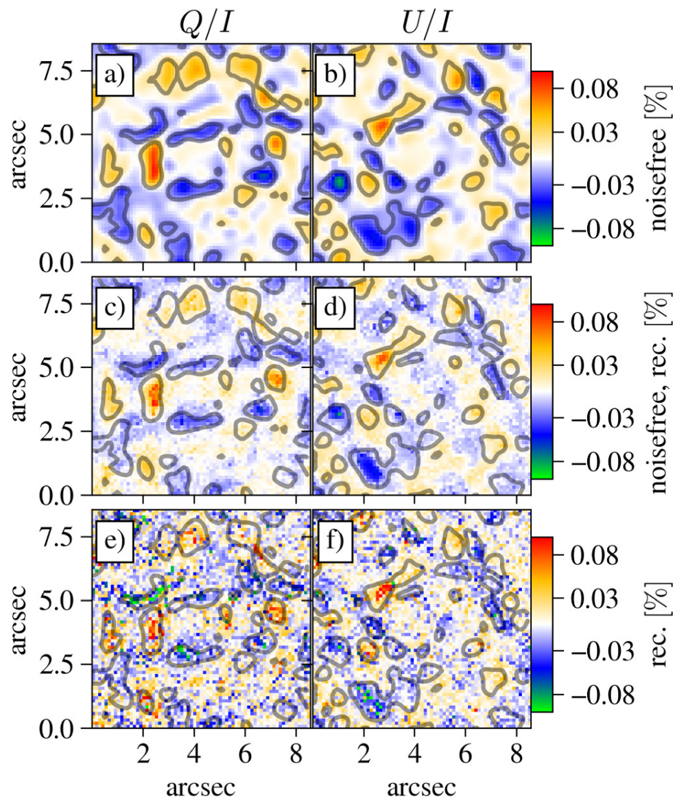
Figure 3. from Franziska Zeuner et al 2024 Astrophys. J. 964 doi:10.3847/1538-4357/ad26f9 https://dx.doi.org/10.3847/1538-4357/ad26f9 © 2024. The Author(s). Published by the American Astronomical Society.
