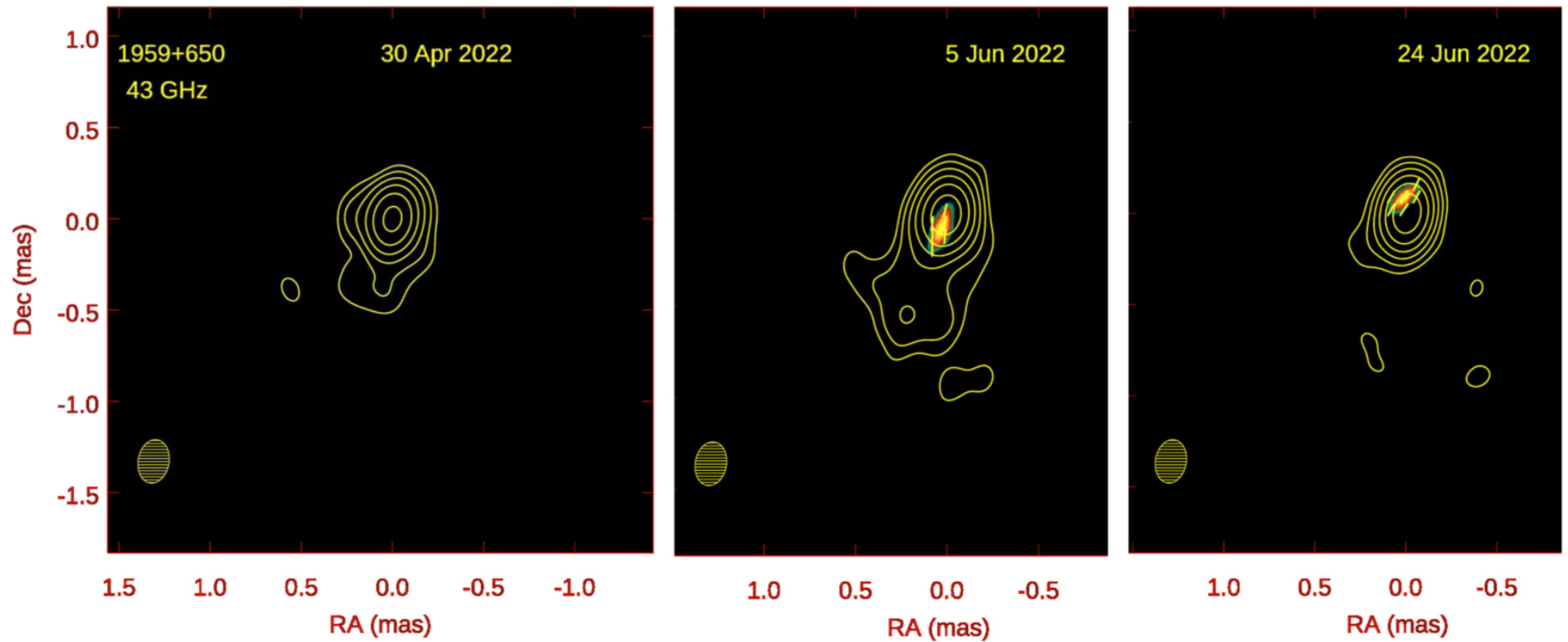
Figure 4. from Manel Errando et al 2024 Astrophys. J. 963 doi:10.3847/1538-4357/ad1ce4 https://dx.doi.org/10.3847/1538-4357/ad1ce4 © 2024. The Author(s). Published by the American Astronomical Society.
