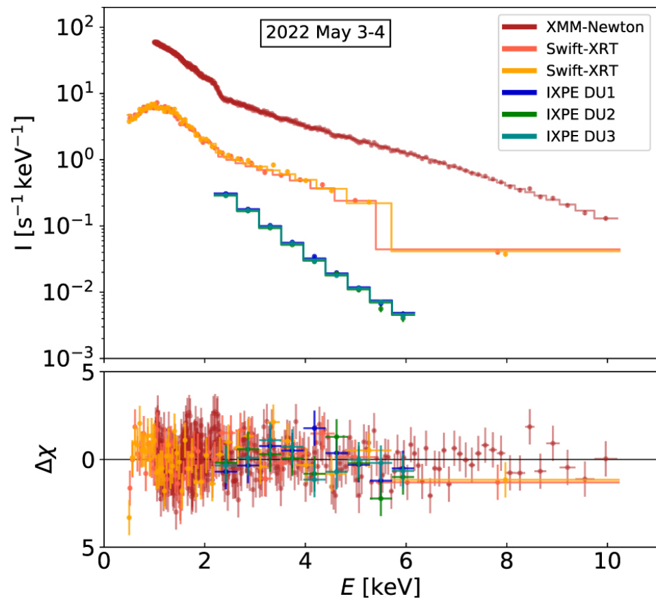
Figure 1. from Manel Errando et al 2024 Astrophys. J. 963 doi:10.3847/1538-4357/ad1ce4 https://dx.doi.org/10.3847/1538-4357/ad1ce4 © 2024. The Author(s). Published by the American Astronomical Society.
