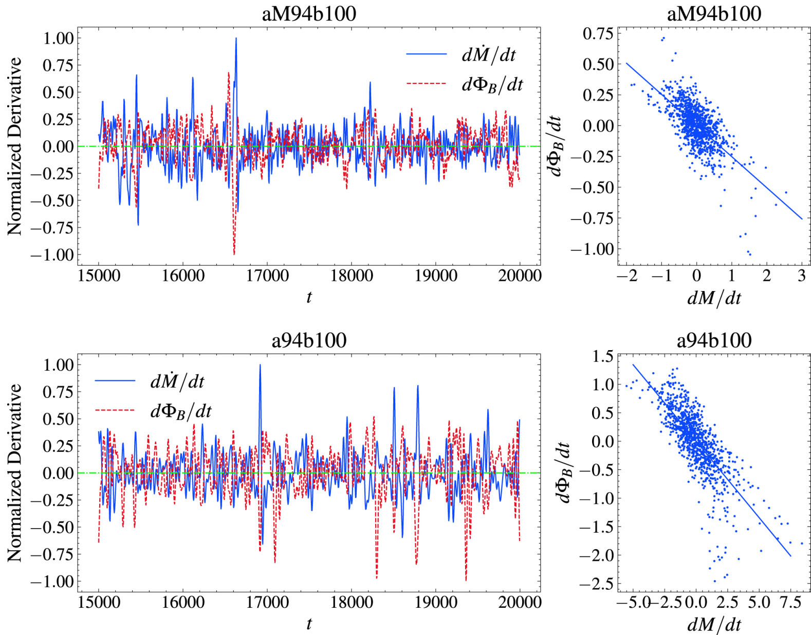
Figure 7. from G.-Q. Zhang et al 2024 Astrophys. J. 962 doi:10.3847/1538-4357/ad167b https://dx.doi.org/10.3847/1538-4357/ad167b © 2024. The Author(s). Published by the American Astronomical Society.
