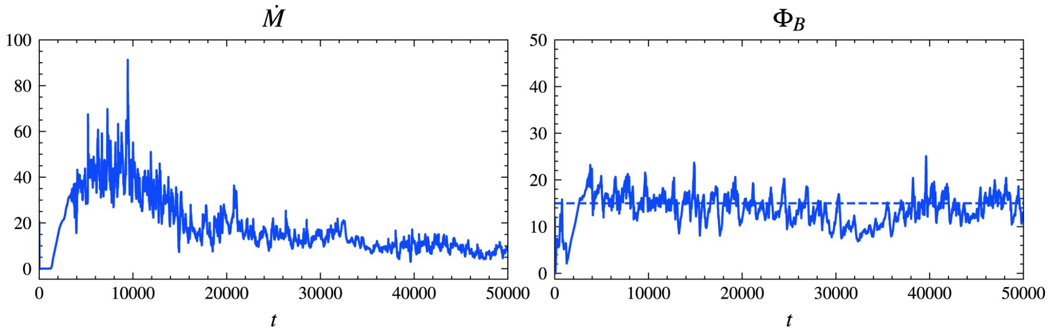
Figure 5. from G.-Q. Zhang et al 2024 Astrophys. J. 962 doi:10.3847/1538-4357/ad167b https://dx.doi.org/10.3847/1538-4357/ad167b © 2024. The Author(s). Published by the American Astronomical Society.
