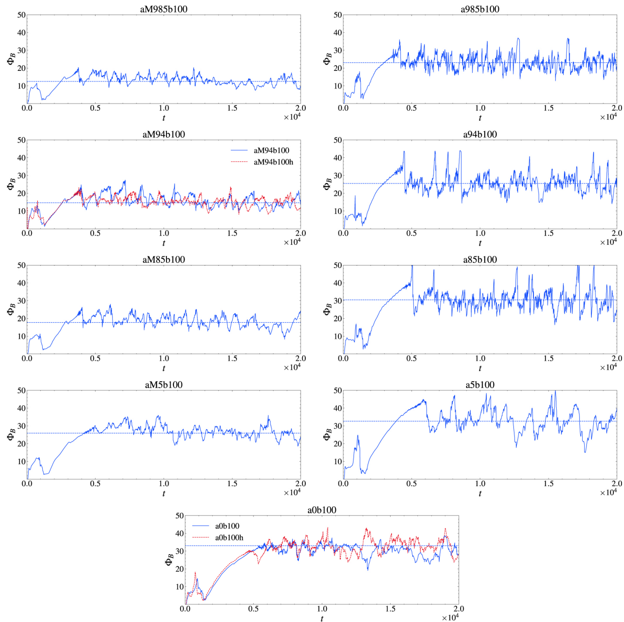
Figure 3. from G.-Q. Zhang et al 2024 Astrophys. J. 962 doi:10.3847/1538-4357/ad167b https://dx.doi.org/10.3847/1538-4357/ad167b © 2024. The Author(s). Published by the American Astronomical Society.
