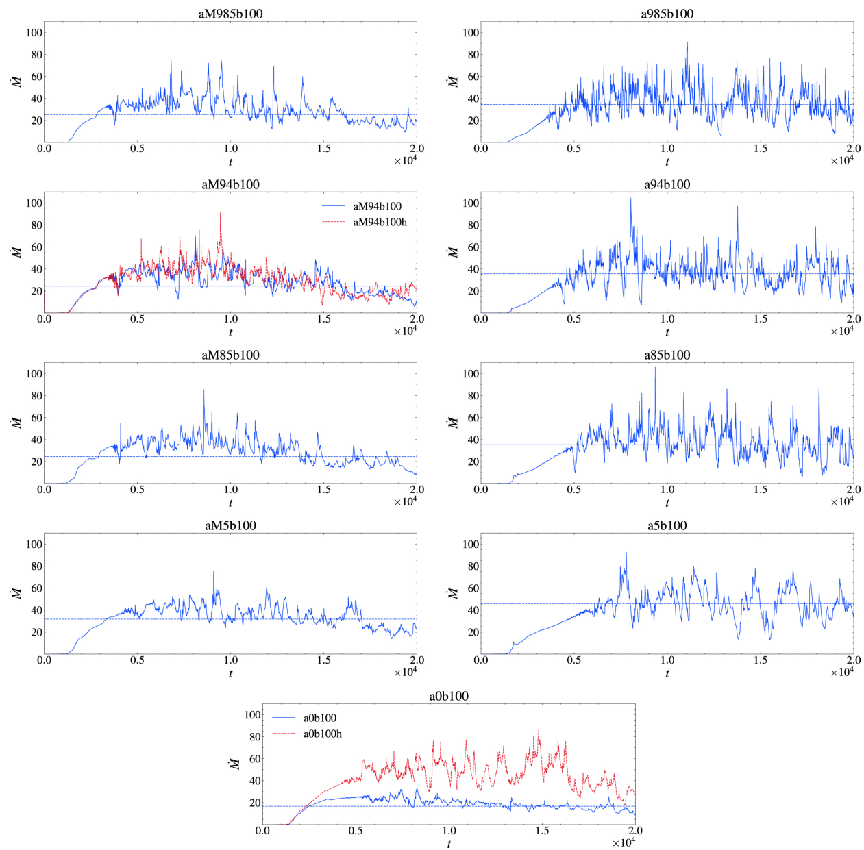
Figure 2. from G.-Q. Zhang et al 2024 Astrophys. J. 962 doi:10.3847/1538-4357/ad167b https://dx.doi.org/10.3847/1538-4357/ad167b © 2024. The Author(s). Published by the American Astronomical Society.
