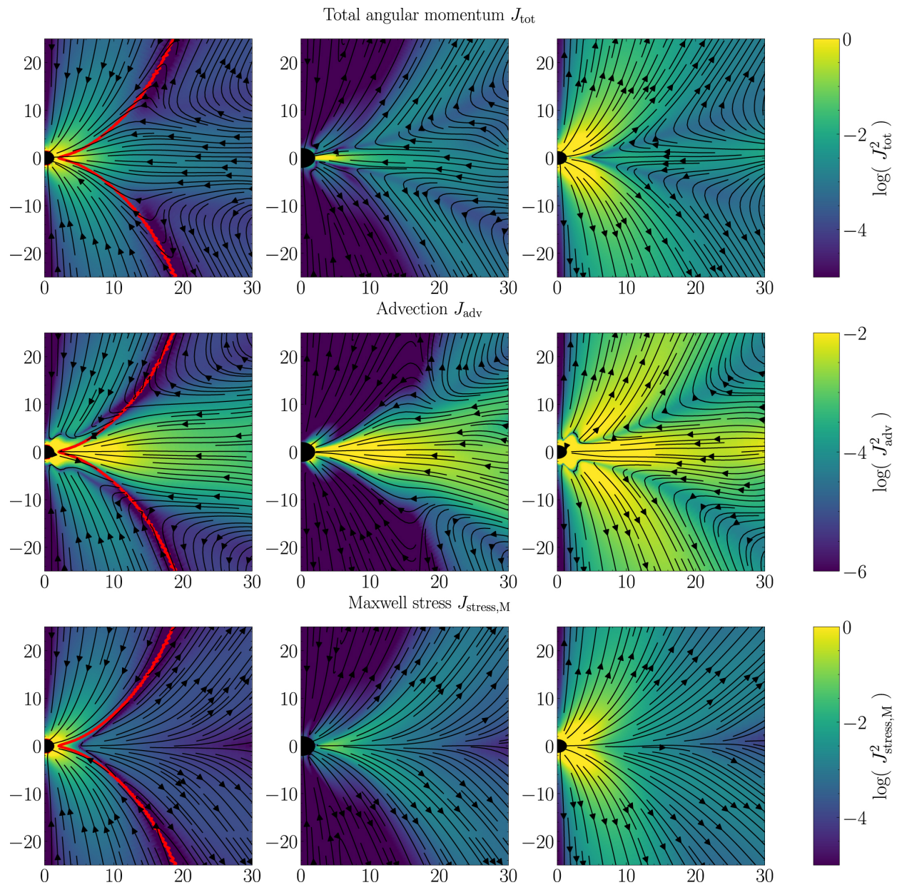
Figure 16. from G.-Q. Zhang et al 2024 Astrophys. J. 962 doi:10.3847/1538-4357/ad167b https://dx.doi.org/10.3847/1538-4357/ad167b © 2024. The Author(s). Published by the American Astronomical Society.
