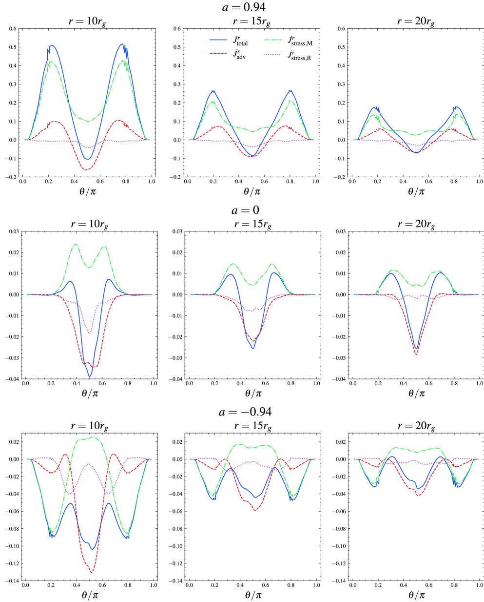
Figure 14. from G.-Q. Zhang et al 2024 Astrophys. J. 962 doi:10.3847/1538-4357/ad167b https://dx.doi.org/10.3847/1538-4357/ad167b © 2024. The Author(s). Published by the American Astronomical Society.
