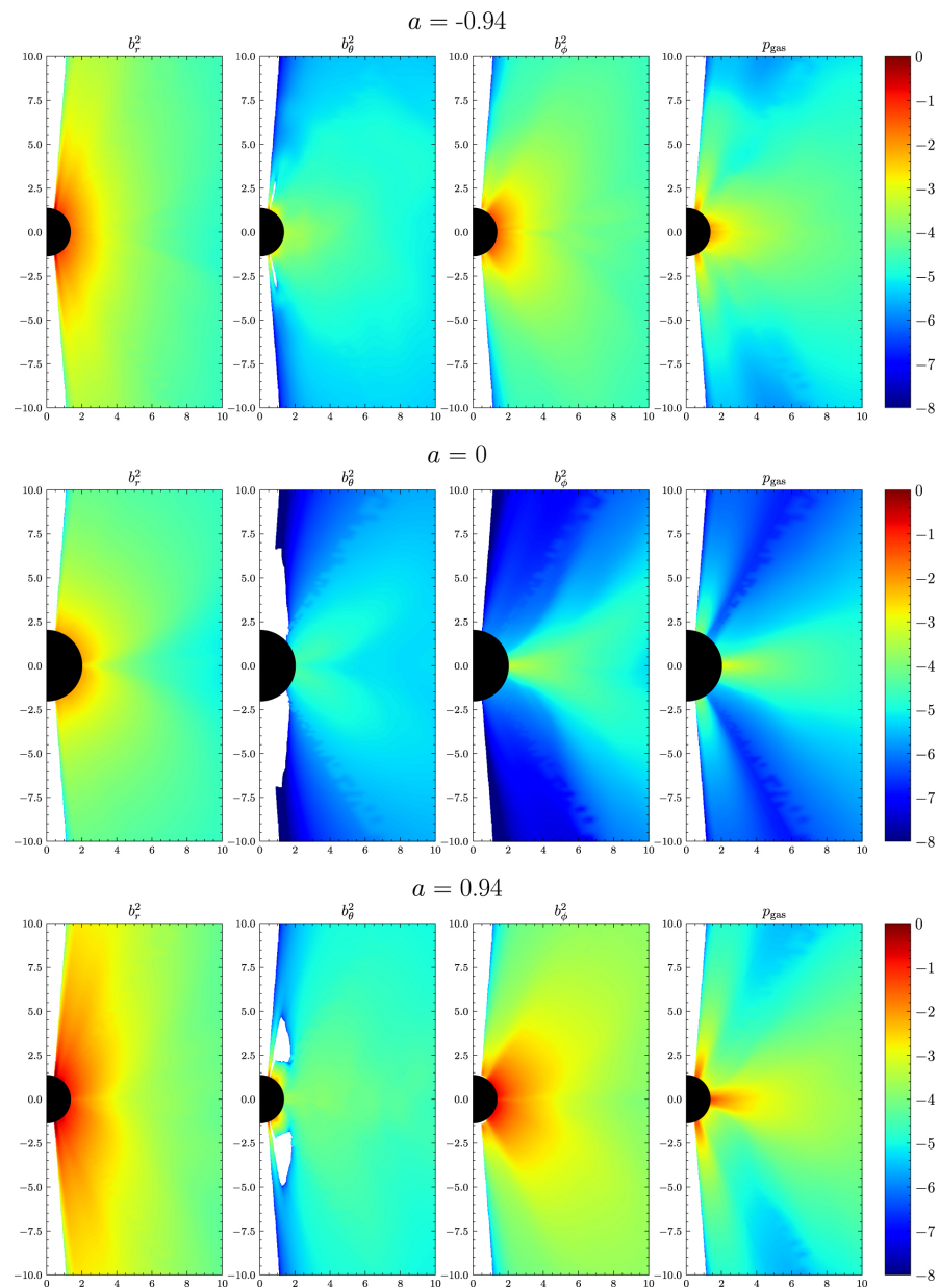
Figure 13. from G.-Q. Zhang et al 2024 Astrophys. J. 962 doi:10.3847/1538-4357/ad167b https://dx.doi.org/10.3847/1538-4357/ad167b © 2024. The Author(s). Published by the American Astronomical Society.
