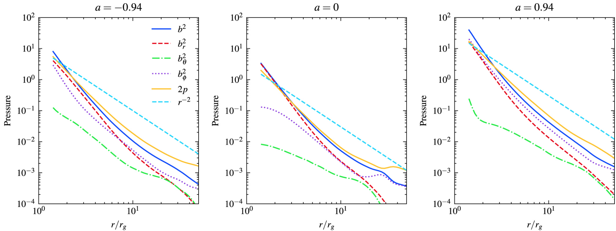
Figure 12. from G.-Q. Zhang et al 2024 Astrophys. J. 962 doi:10.3847/1538-4357/ad167b https://dx.doi.org/10.3847/1538-4357/ad167b © 2024. The Author(s). Published by the American Astronomical Society.
