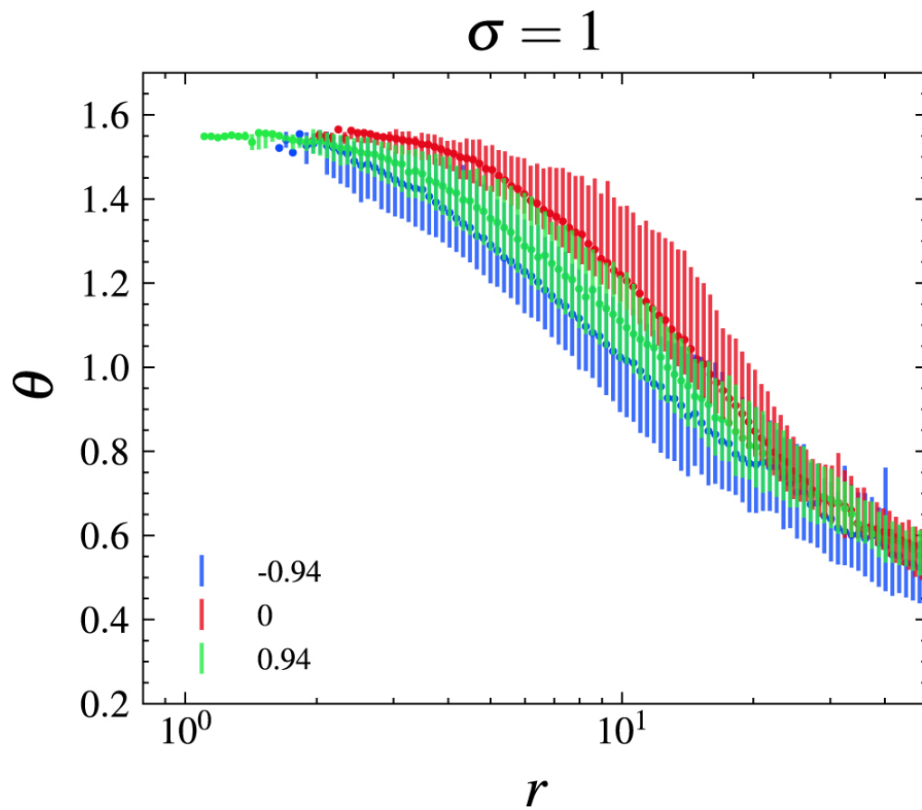
Figure 11. from G.-Q. Zhang et al 2024 Astrophys. J. 962 doi:10.3847/1538-4357/ad167b https://dx.doi.org/10.3847/1538-4357/ad167b © 2024. The Author(s). Published by the American Astronomical Society.
