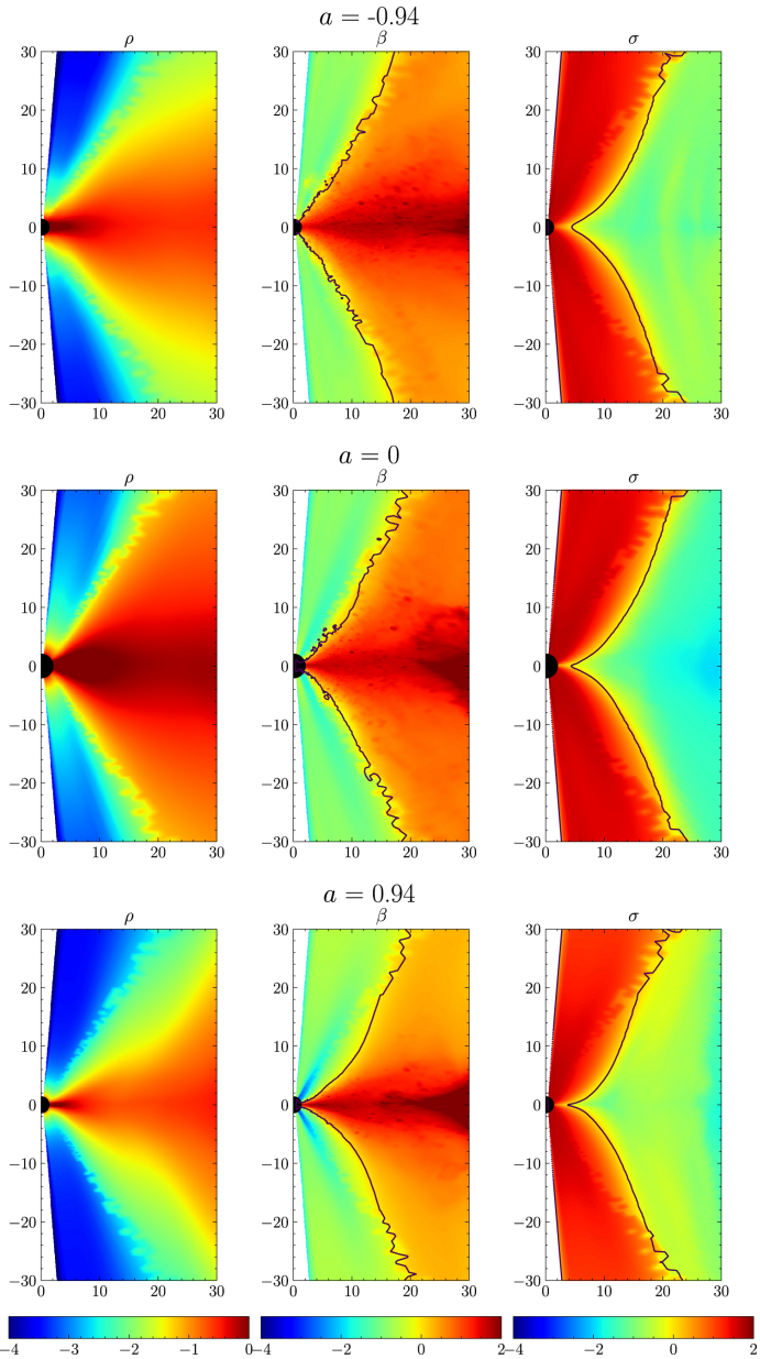
Figure 10. from G.-Q. Zhang et al 2024 Astrophys. J. 962 doi:10.3847/1538-4357/ad167b https://dx.doi.org/10.3847/1538-4357/ad167b © 2024. The Author(s). Published by the American Astronomical Society.
