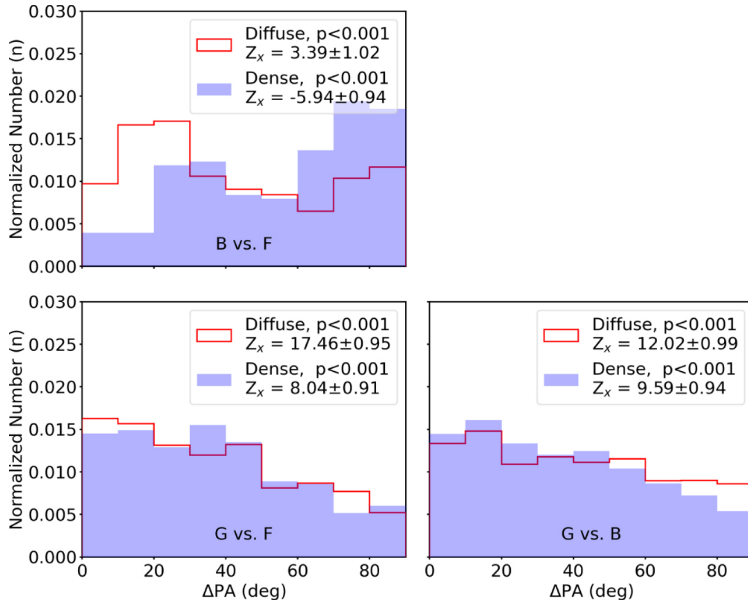
Figure 8. from Jia-Wei Wang et al 2024 Astrophys. J. 962 doi:10.3847/1538-4357/ad165b https://dx.doi.org/10.3847/1538-4357/ad165b © 2024. The Author(s). Published by the American Astronomical Society.
