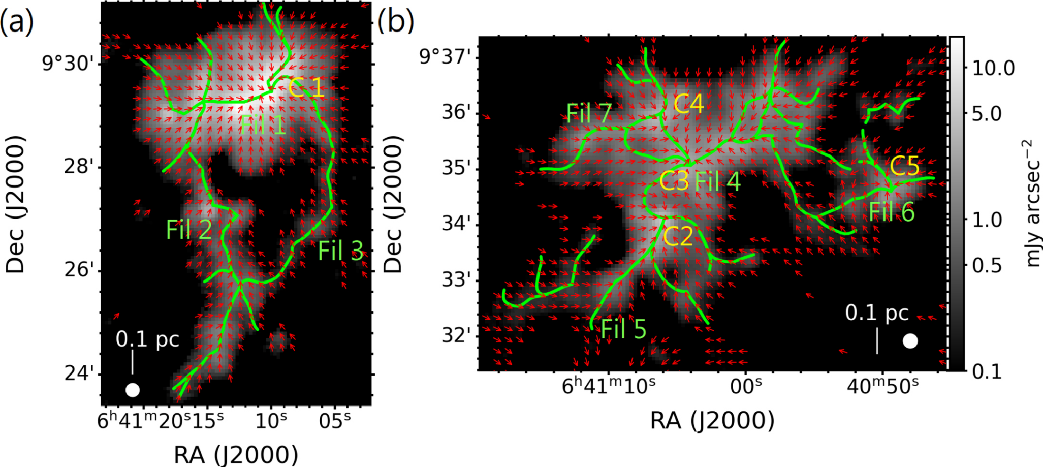
Figure 6. from Jia-Wei Wang et al 2024 Astrophys. J. 962 doi:10.3847/1538-4357/ad165b https://dx.doi.org/10.3847/1538-4357/ad165b © 2024. The Author(s). Published by the American Astronomical Society.
