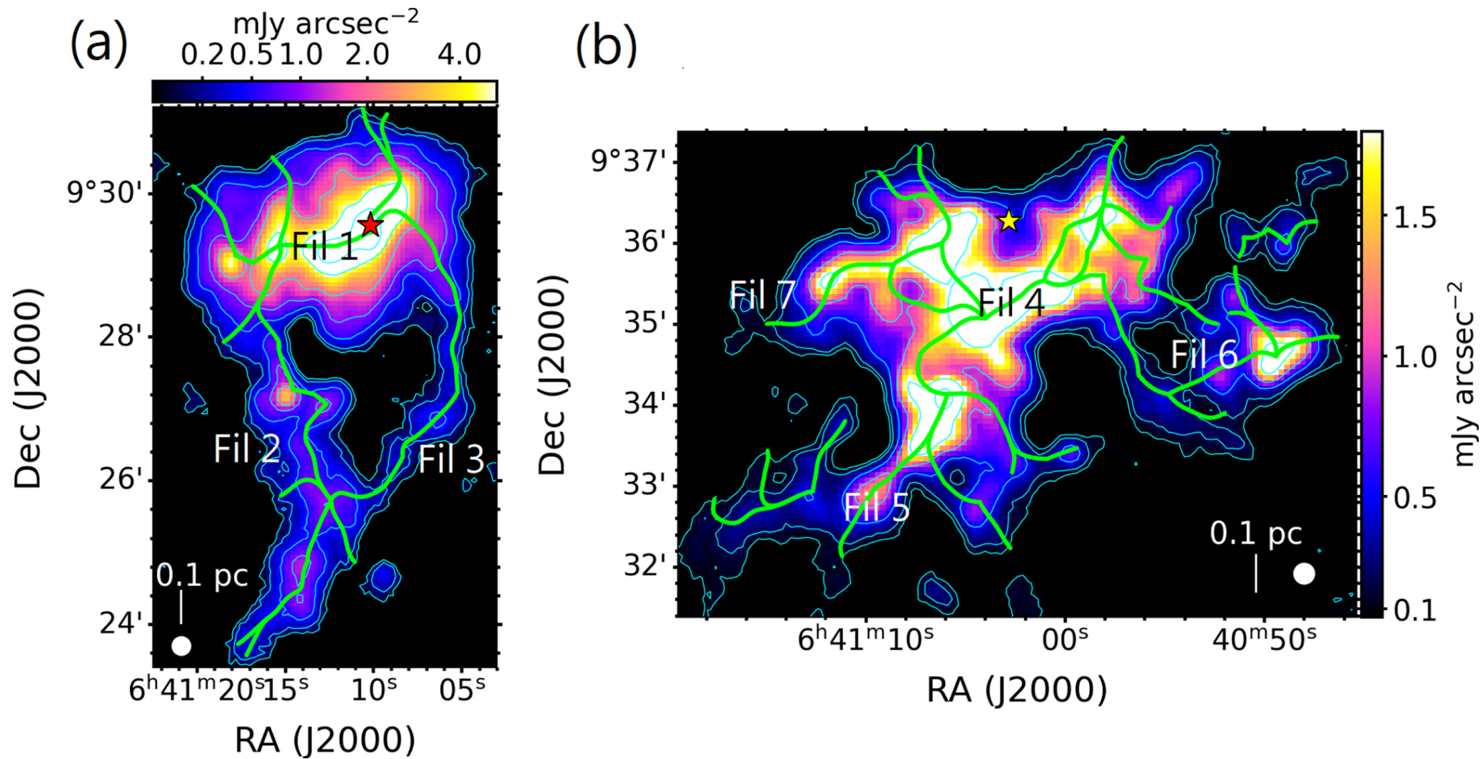
Figure 5. from Jia-Wei Wang et al 2024 Astrophys. J. 962 doi:10.3847/1538-4357/ad165b https://dx.doi.org/10.3847/1538-4357/ad165b © 2024. The Author(s). Published by the American Astronomical Society.
