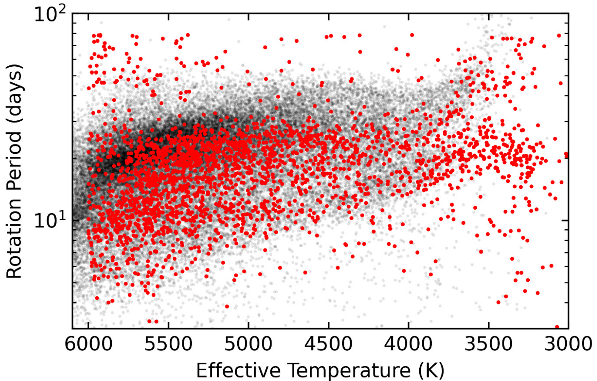
Figure 8. from Zachary R. Claytor et al 2024 Astrophys. J. 962 doi:10.3847/1538-4357/ad159a https://dx.doi.org/10.3847/1538-4357/ad159a © 2024. The Author(s). Published by the American Astronomical Society.
