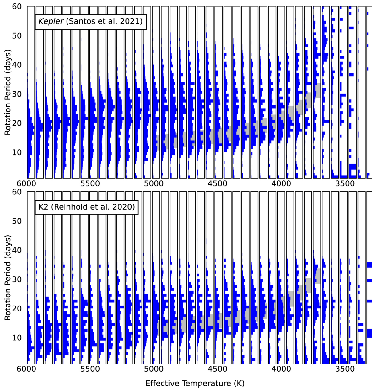
Figure 6. from Zachary R. Claytor et al 2024 Astrophys. J. 962 doi:10.3847/1538-4357/ad159a https://dx.doi.org/10.3847/1538-4357/ad159a © 2024. The Author(s). Published by the American Astronomical Society.
