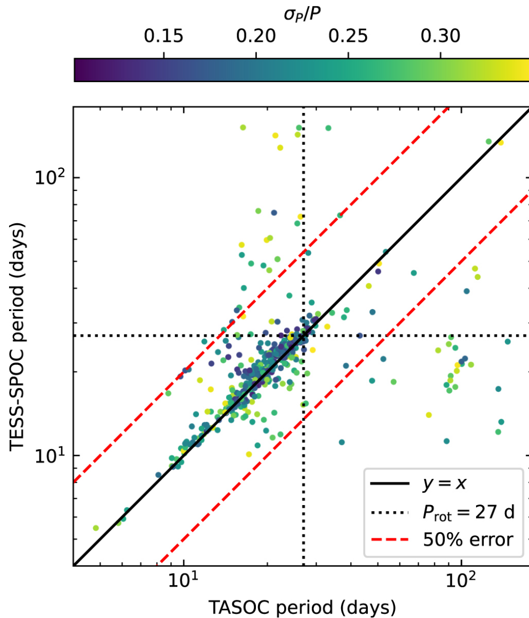
Figure 5. from Zachary R. Claytor et al 2024 Astrophys. J. 962 doi:10.3847/1538-4357/ad159a https://dx.doi.org/10.3847/1538-4357/ad159a © 2024. The Author(s). Published by the American Astronomical Society.
