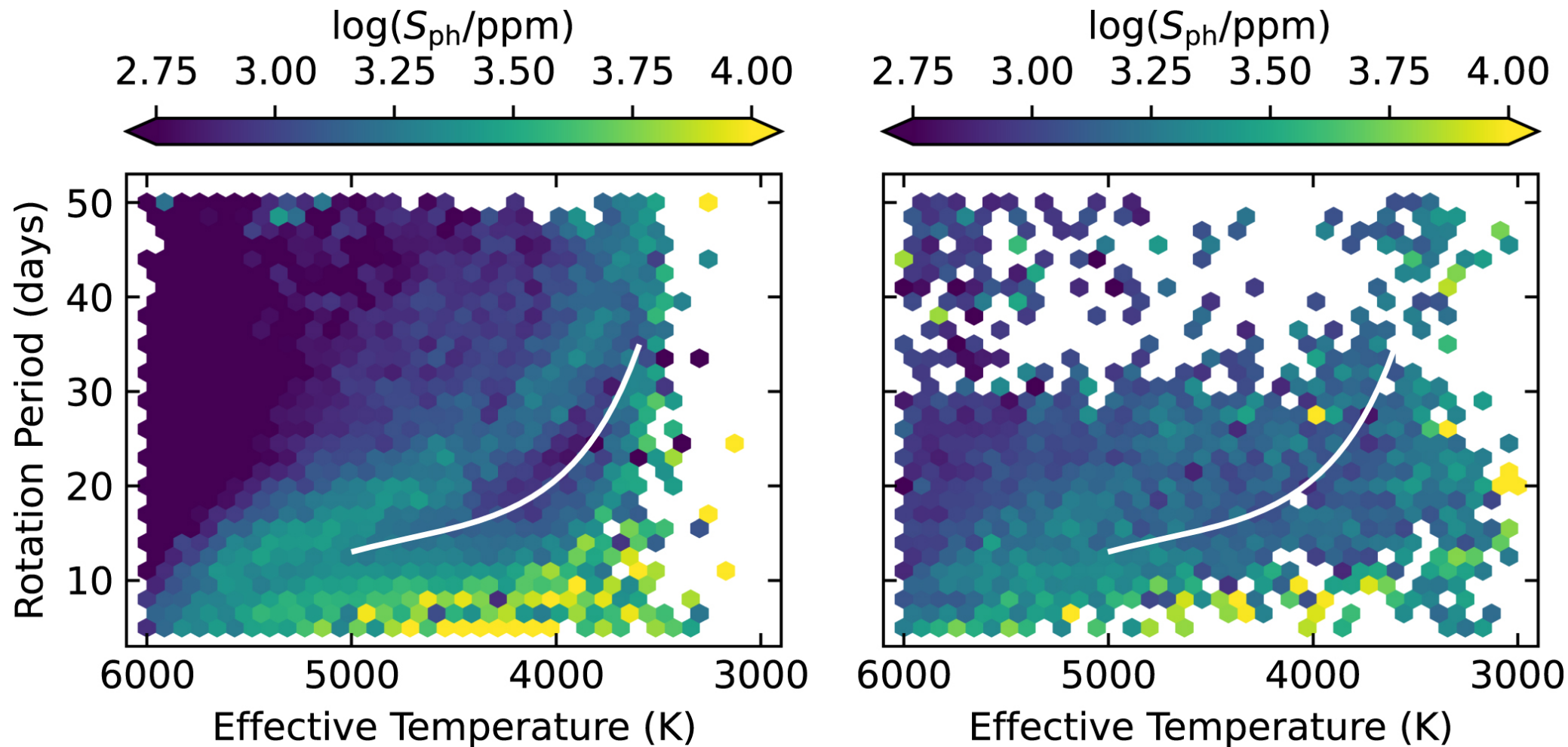
Figure 3. from Zachary R. Claytor et al 2024 Astrophys. J. 962 doi:10.3847/1538-4357/ad159a https://dx.doi.org/10.3847/1538-4357/ad159a © 2024. The Author(s). Published by the American Astronomical Society.
