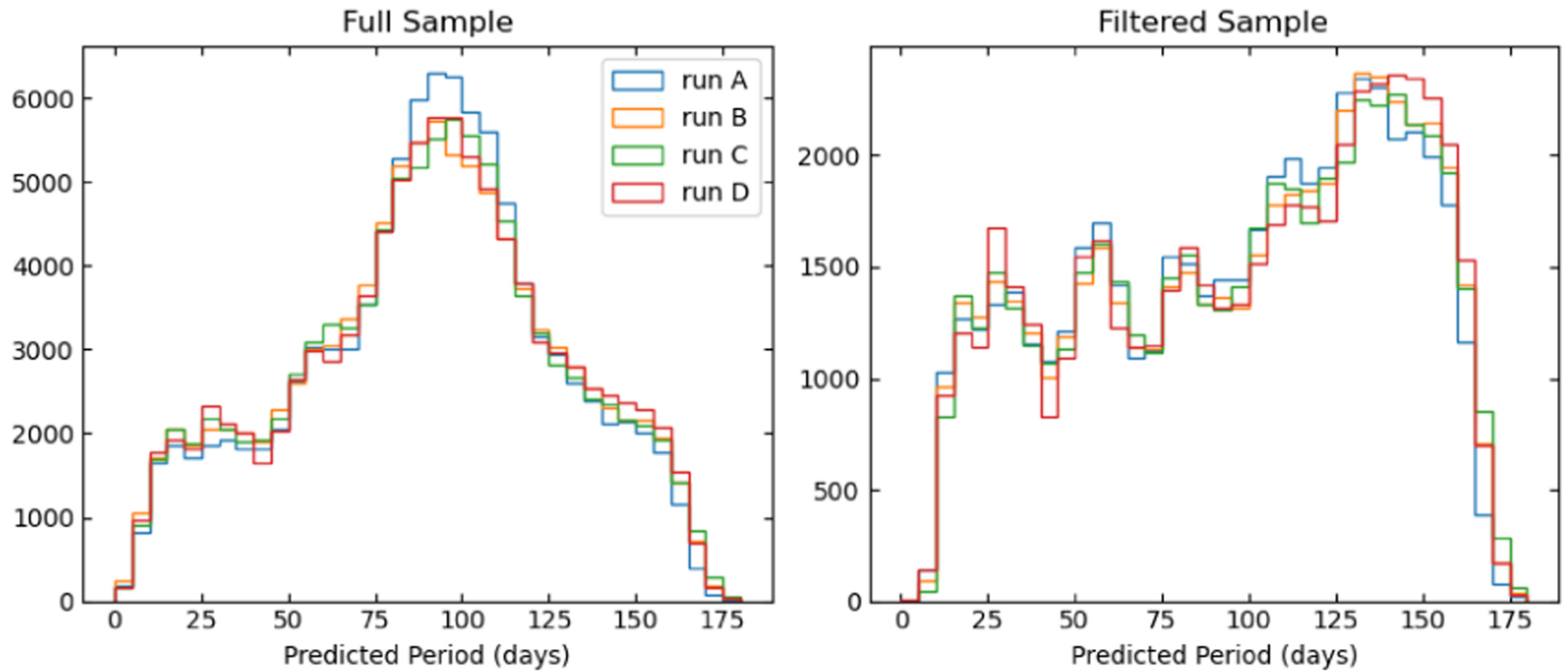
Figure 22. from Zachary R. Claytor et al 2024 Astrophys. J. 962 doi:10.3847/1538-4357/ad159a https://dx.doi.org/10.3847/1538-4357/ad159a © 2024. The Author(s). Published by the American Astronomical Society.
