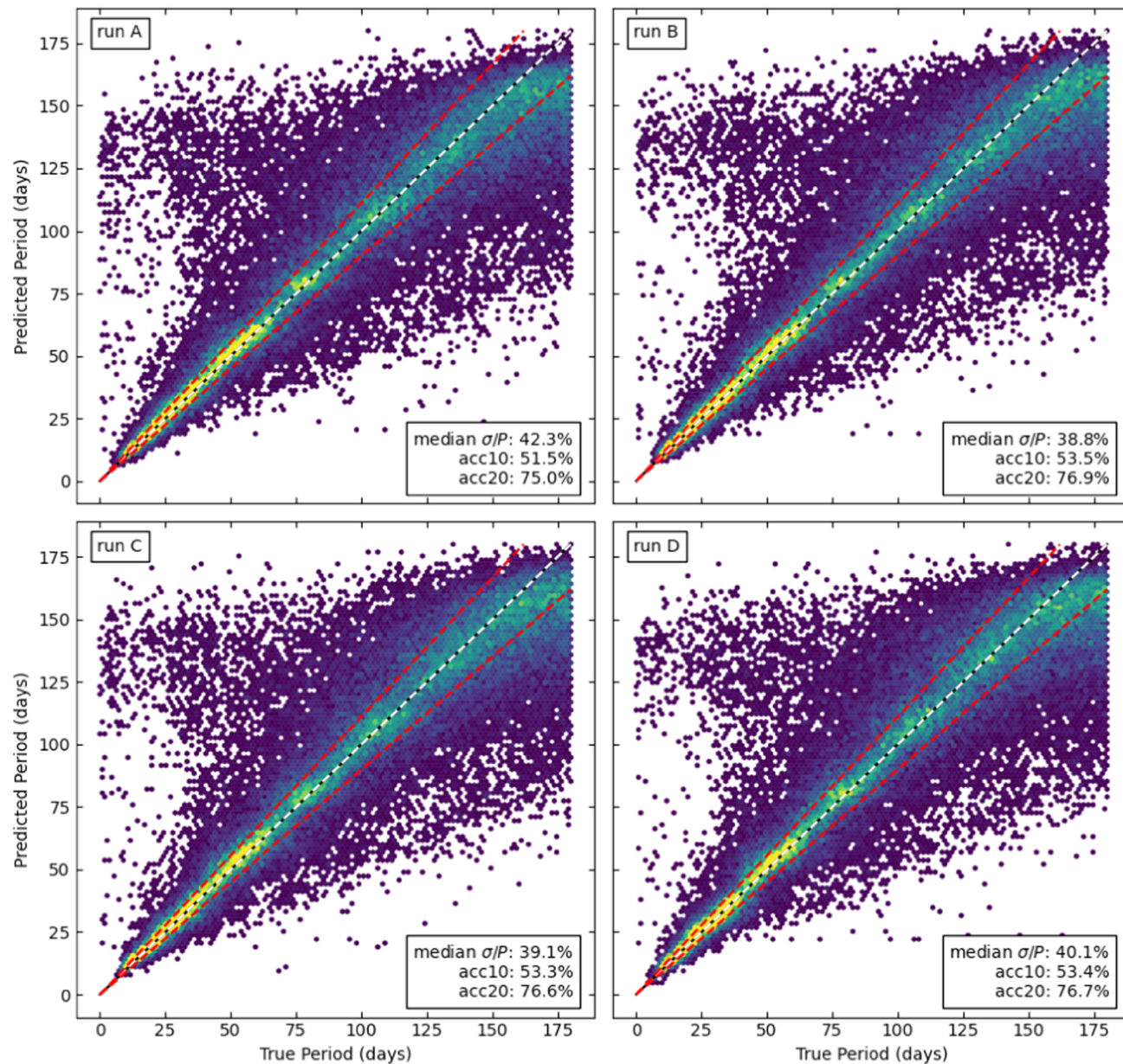
Figure 21. from Zachary R. Claytor et al 2024 Astrophys. J. 962 doi:10.3847/1538-4357/ad159a https://dx.doi.org/10.3847/1538-4357/ad159a © 2024. The Author(s). Published by the American Astronomical Society.
