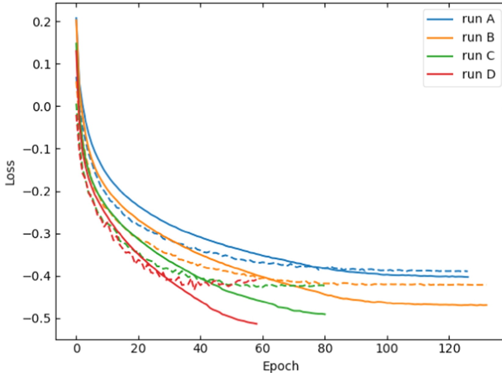
Figure 20. from Zachary R. Claytor et al 2024 Astrophys. J. 962 doi:10.3847/1538-4357/ad159a https://dx.doi.org/10.3847/1538-4357/ad159a © 2024. The Author(s). Published by the American Astronomical Society.
