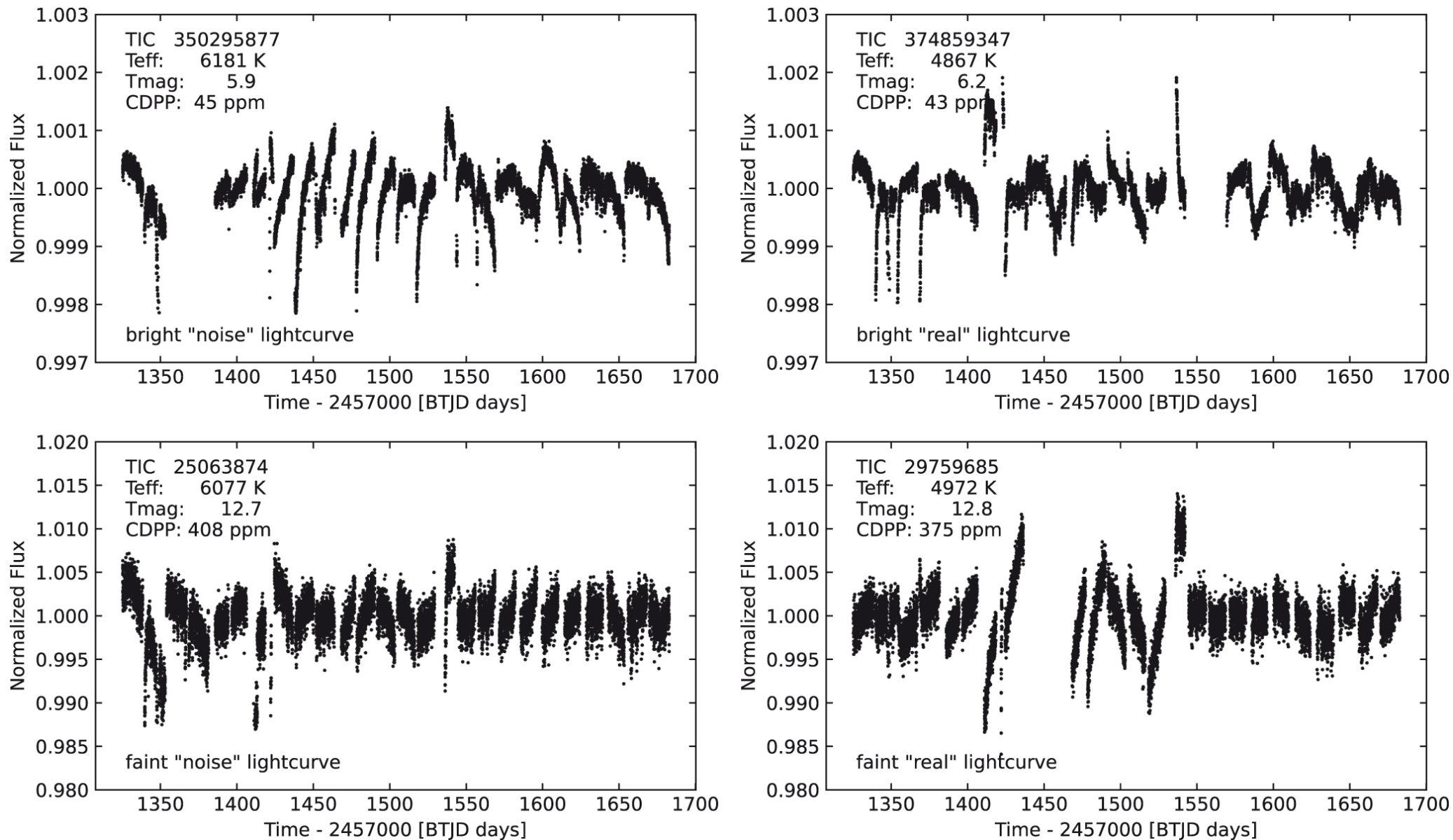
Figure 19. from Zachary R. Claytor et al 2024 Astrophys. J. 962 doi:10.3847/1538-4357/ad159a https://dx.doi.org/10.3847/1538-4357/ad159a
