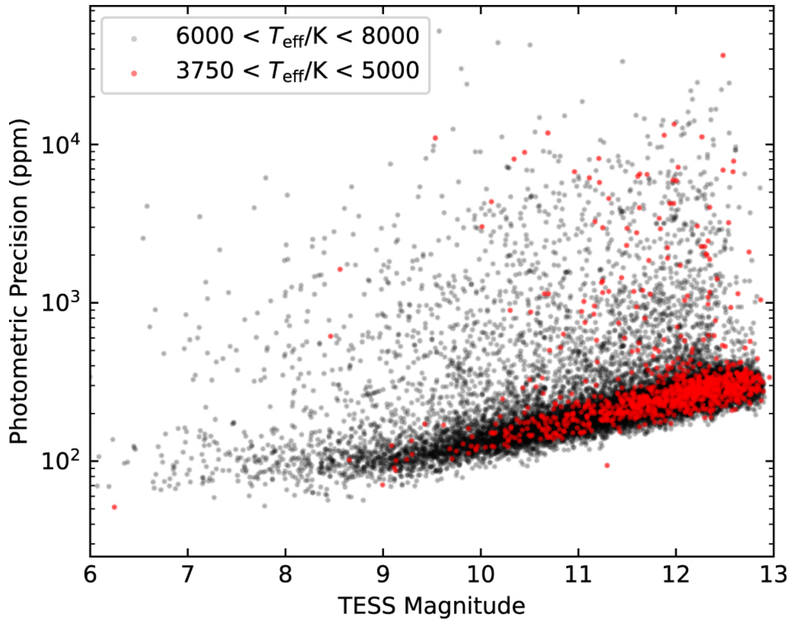
Figure 18. from Zachary R. Claytor et al 2024 Astrophys. J. 962 doi:10.3847/1538-4357/ad159a https://dx.doi.org/10.3847/1538-4357/ad159a © 2024. The Author(s). Published by the American Astronomical Society.
