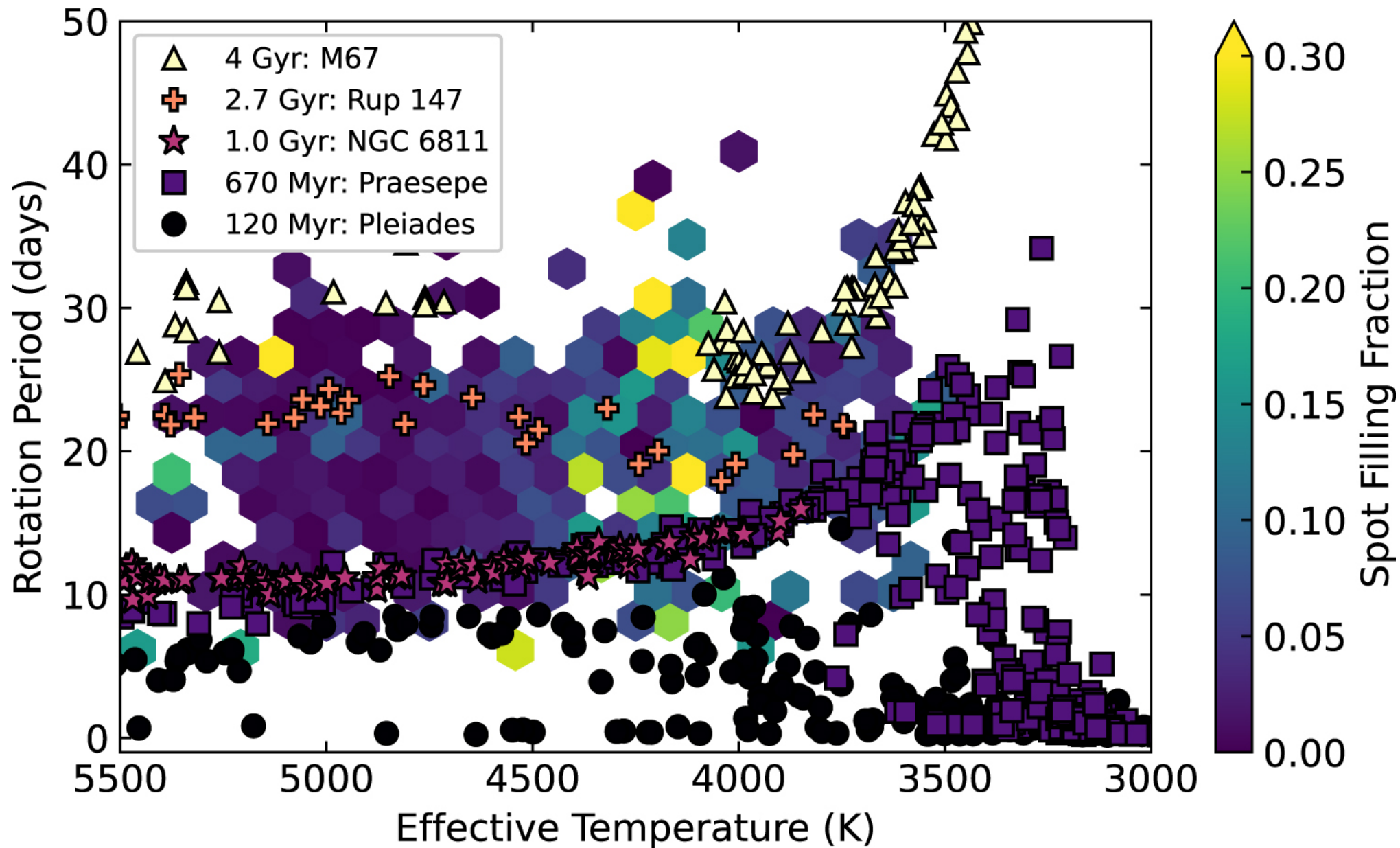
Figure 17. from Zachary R. Claytor et al 2024 Astrophys. J. 962 doi:10.3847/1538-4357/ad159a https://dx.doi.org/10.3847/1538-4357/ad159a © 2024. The Author(s). Published by the American Astronomical Society.
