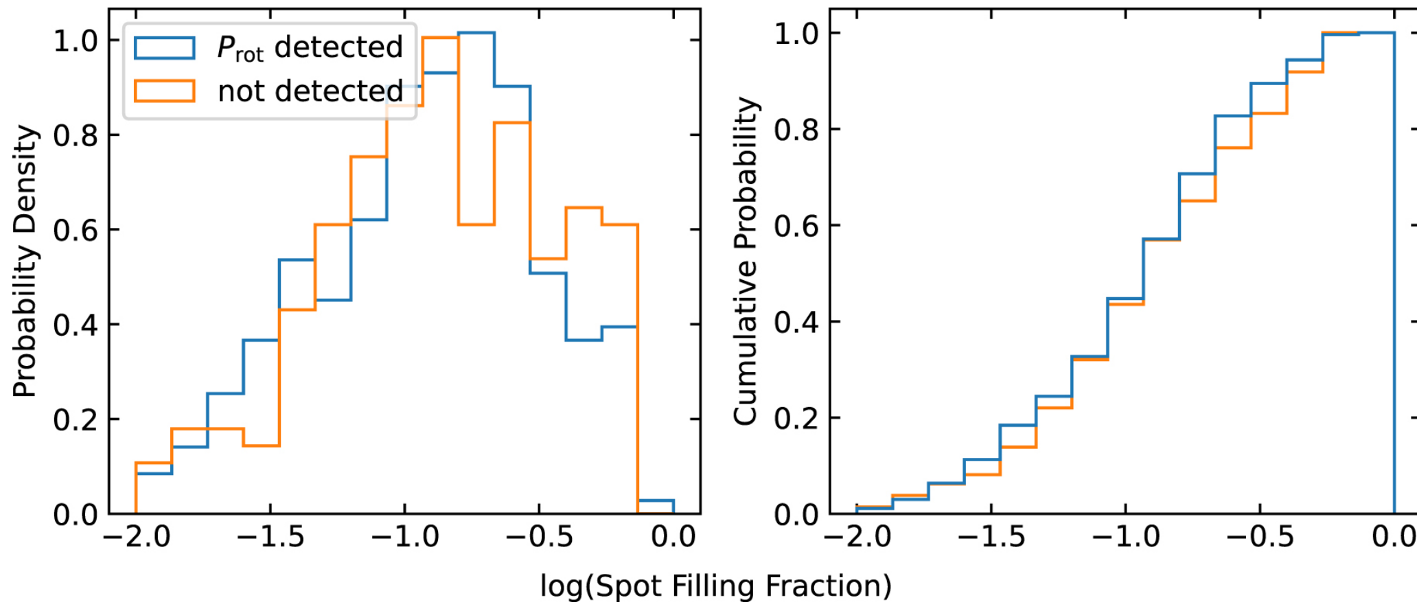
Figure 16. from Zachary R. Claytor et al 2024 Astrophys. J. 962 doi:10.3847/1538-4357/ad159a https://dx.doi.org/10.3847/1538-4357/ad159a © 2024. The Author(s). Published by the American Astronomical Society.
