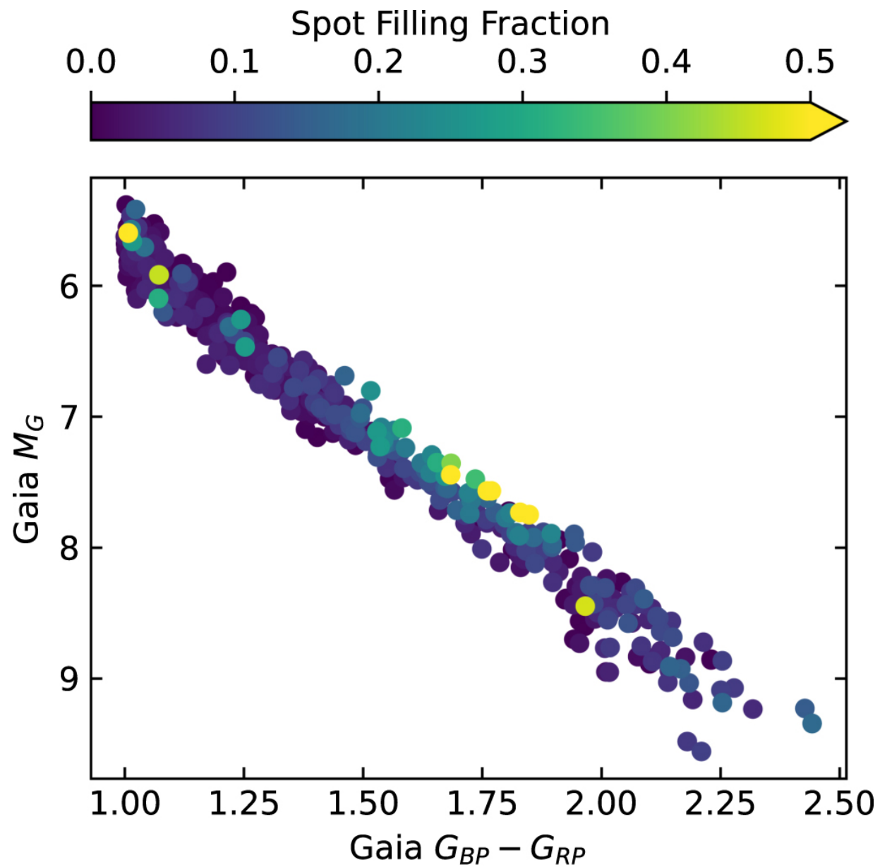
Figure 15. from Zachary R. Claytor et al 2024 Astrophys. J. 962 doi:10.3847/1538-4357/ad159a https://dx.doi.org/10.3847/1538-4357/ad159a © 2024. The Author(s). Published by the American Astronomical Society.
