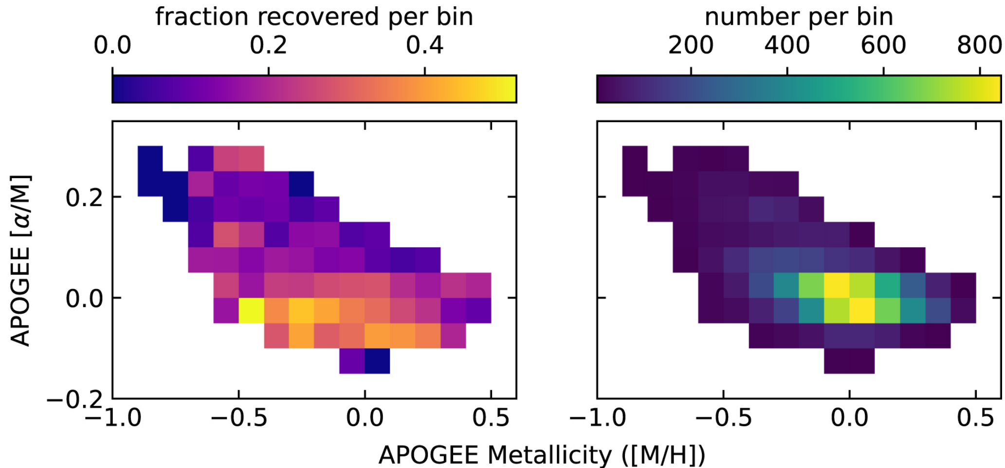
Figure 14. from Zachary R. Claytor et al 2024 Astrophys. J. 962 doi:10.3847/1538-4357/ad159a https://dx.doi.org/10.3847/1538-4357/ad159a © 2024. The Author(s). Published by the American Astronomical Society.
