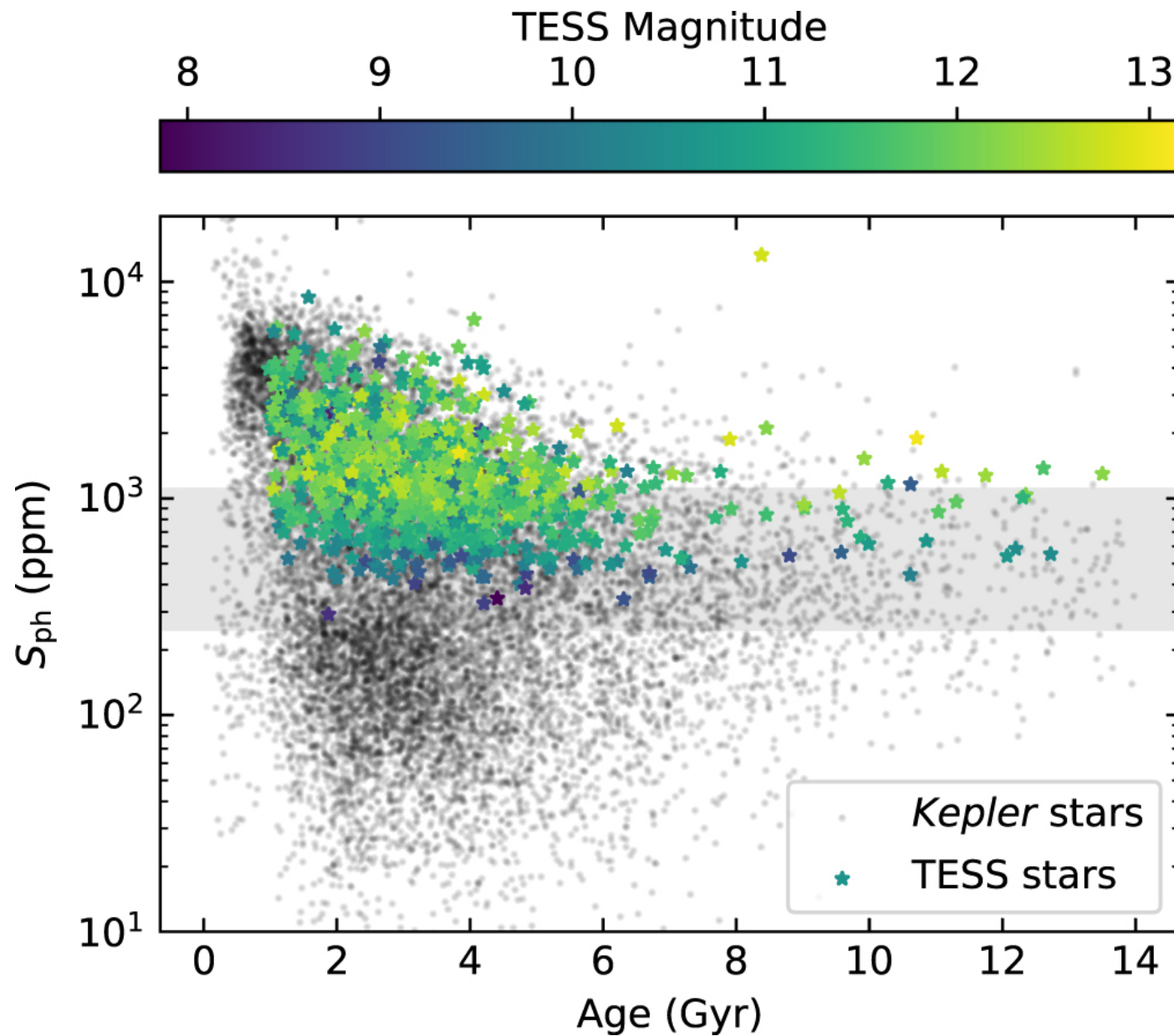
Figure 12. from Zachary R. Claytor et al 2024 Astrophys. J. 962 doi:10.3847/1538-4357/ad159a https://dx.doi.org/10.3847/1538-4357/ad159a © 2024. The Author(s). Published by the American Astronomical Society.
