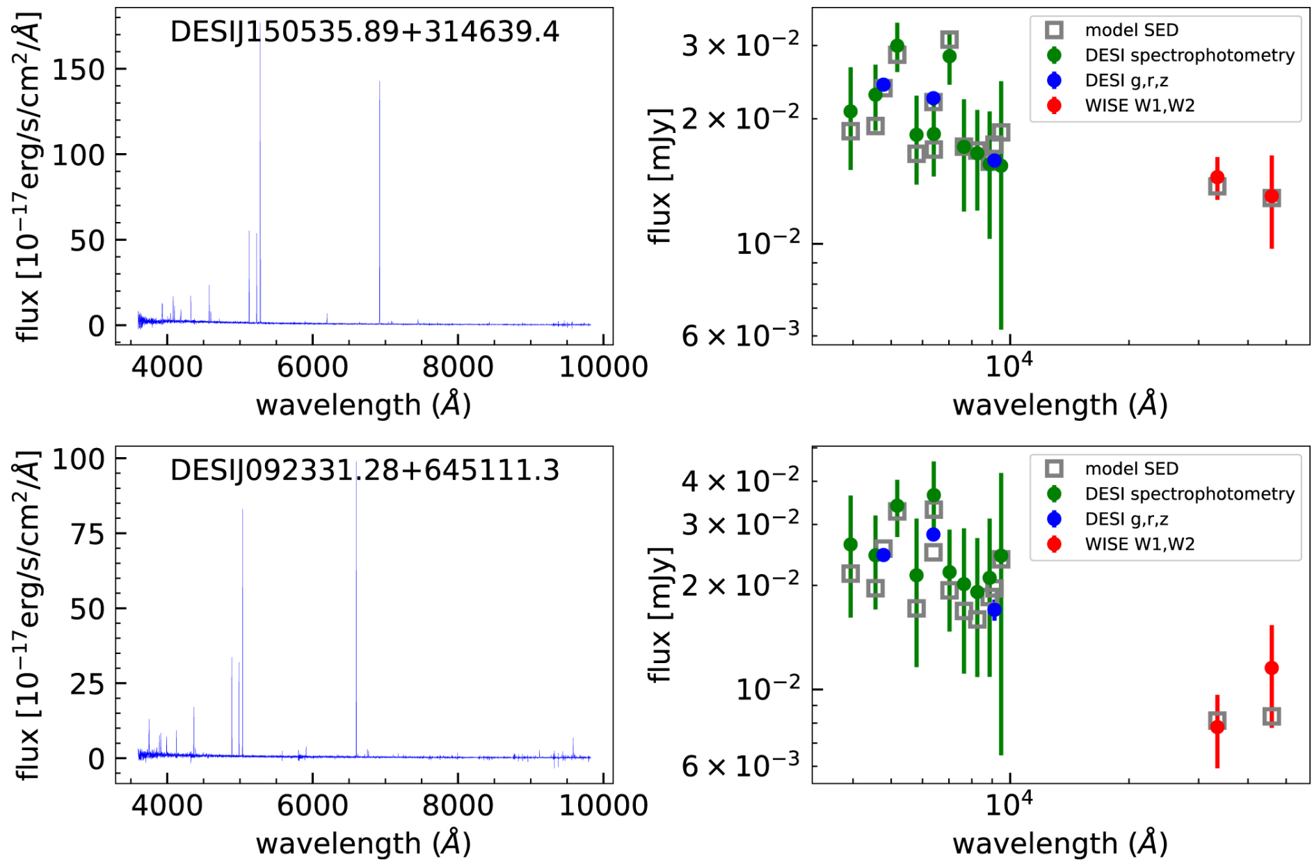
Figure 9. from Hu Zou et al 2024 Astrophys. J. 961 doi:10.3847/1538-4357/ad1409 https://dx.doi.org/10.3847/1538-4357/ad1409 © 2024. The Author(s). Published by the American Astronomical Society.
