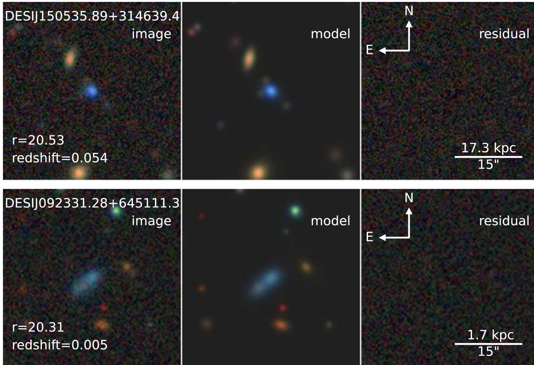
Figure 8. from Hu Zou et al 2024 Astrophys. J. 961 doi:10.3847/1538-4357/ad1409 https://dx.doi.org/10.3847/1538-4357/ad1409 © 2024. The Author(s). Published by the American Astronomical Society.
