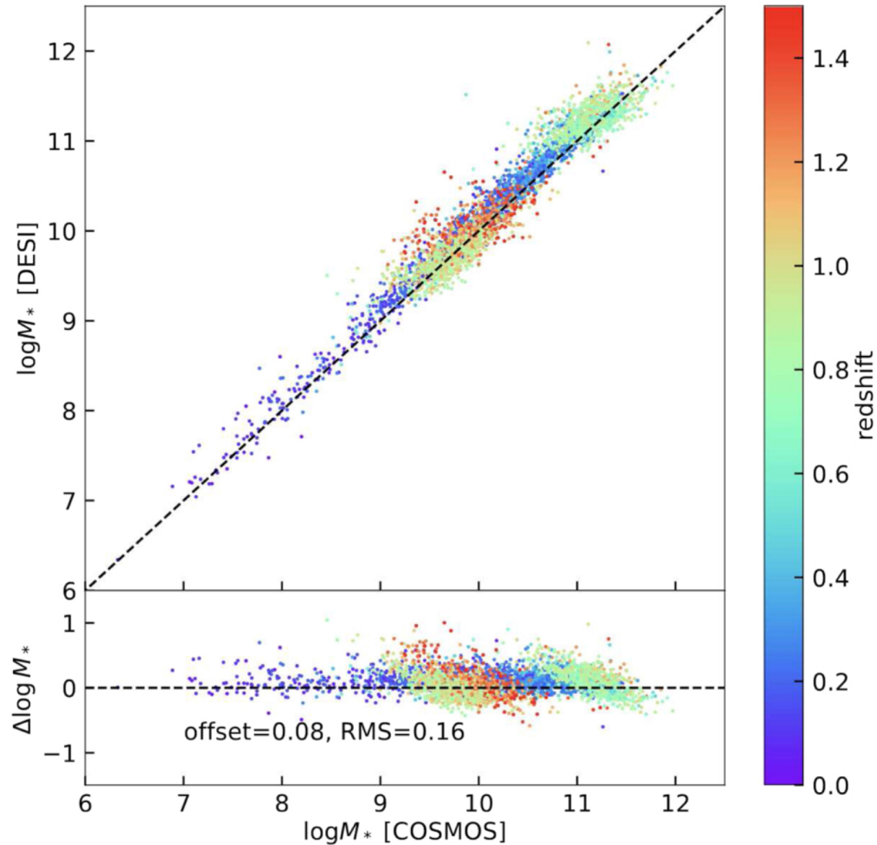
Figure 6. from Hu Zou et al 2024 Astrophys. J. 961 doi:10.3847/1538-4357/ad1409 https://dx.doi.org/10.3847/1538-4357/ad1409 © 2024. The Author(s). Published by the American Astronomical Society.
