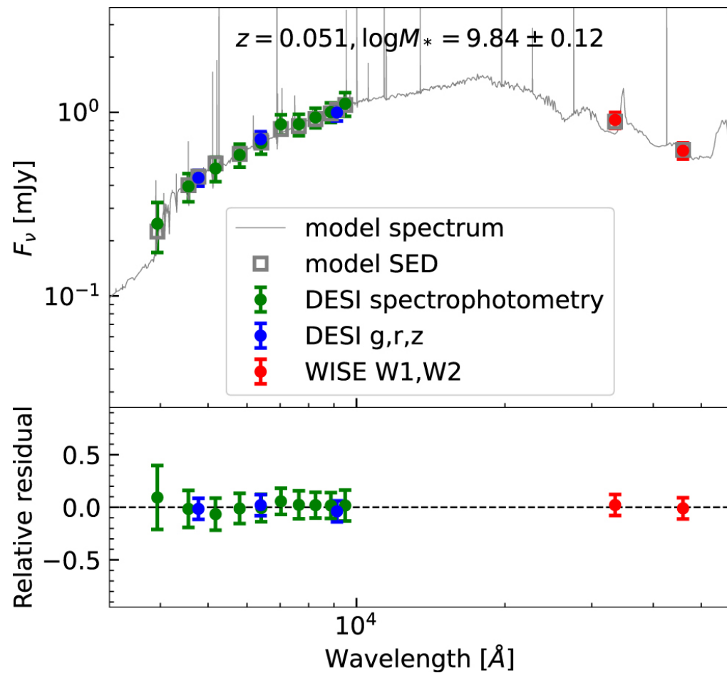
Figure 5. from Hu Zou et al 2024 Astrophys. J. 961 doi:10.3847/1538-4357/ad1409 https://dx.doi.org/10.3847/1538-4357/ad1409 © 2024. The Author(s). Published by the American Astronomical Society.
