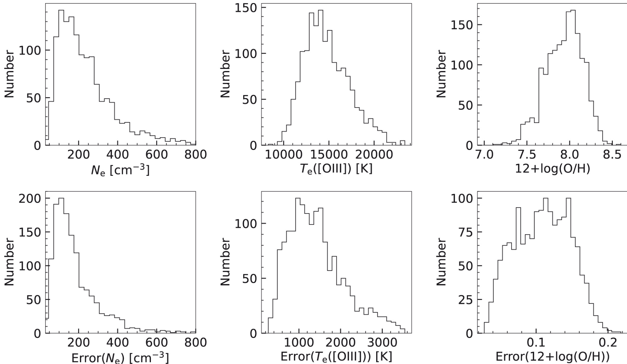
Figure 4. from Hu Zou et al 2024 Astrophys. J. 961 doi:10.3847/1538-4357/ad1409 https://dx.doi.org/10.3847/1538-4357/ad1409 © 2024. The Author(s). Published by the American Astronomical Society.
