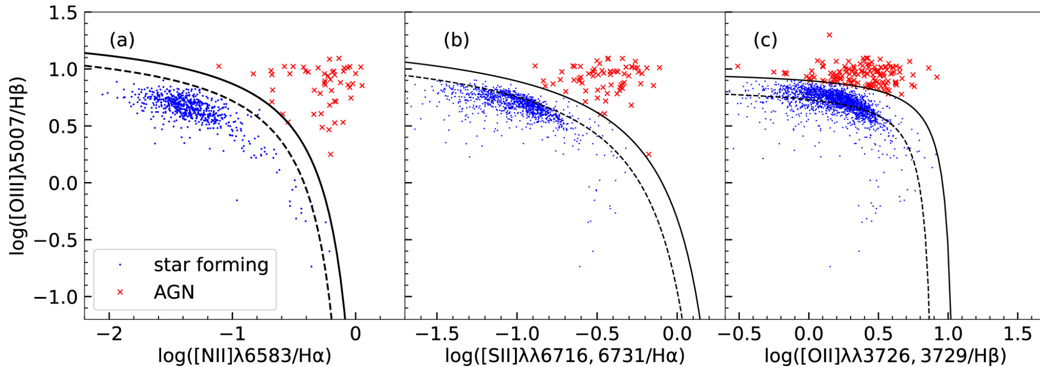
Figure 3. from Hu Zou et al 2024 Astrophys. J. 961 doi:10.3847/1538-4357/ad1409 https://dx.doi.org/10.3847/1538-4357/ad1409 © 2024. The Author(s). Published by the American Astronomical Society.
