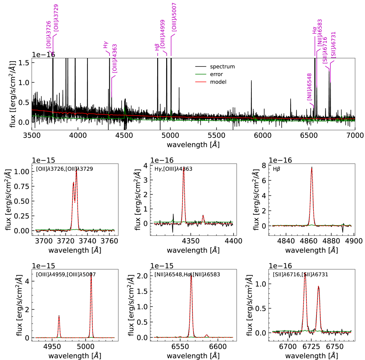
Figure 2. from Hu Zou et al 2024 Astrophys. J. 961 doi:10.3847/1538-4357/ad1409 https://dx.doi.org/10.3847/1538-4357/ad1409 © 2024. The Author(s). Published by the American Astronomical Society.
