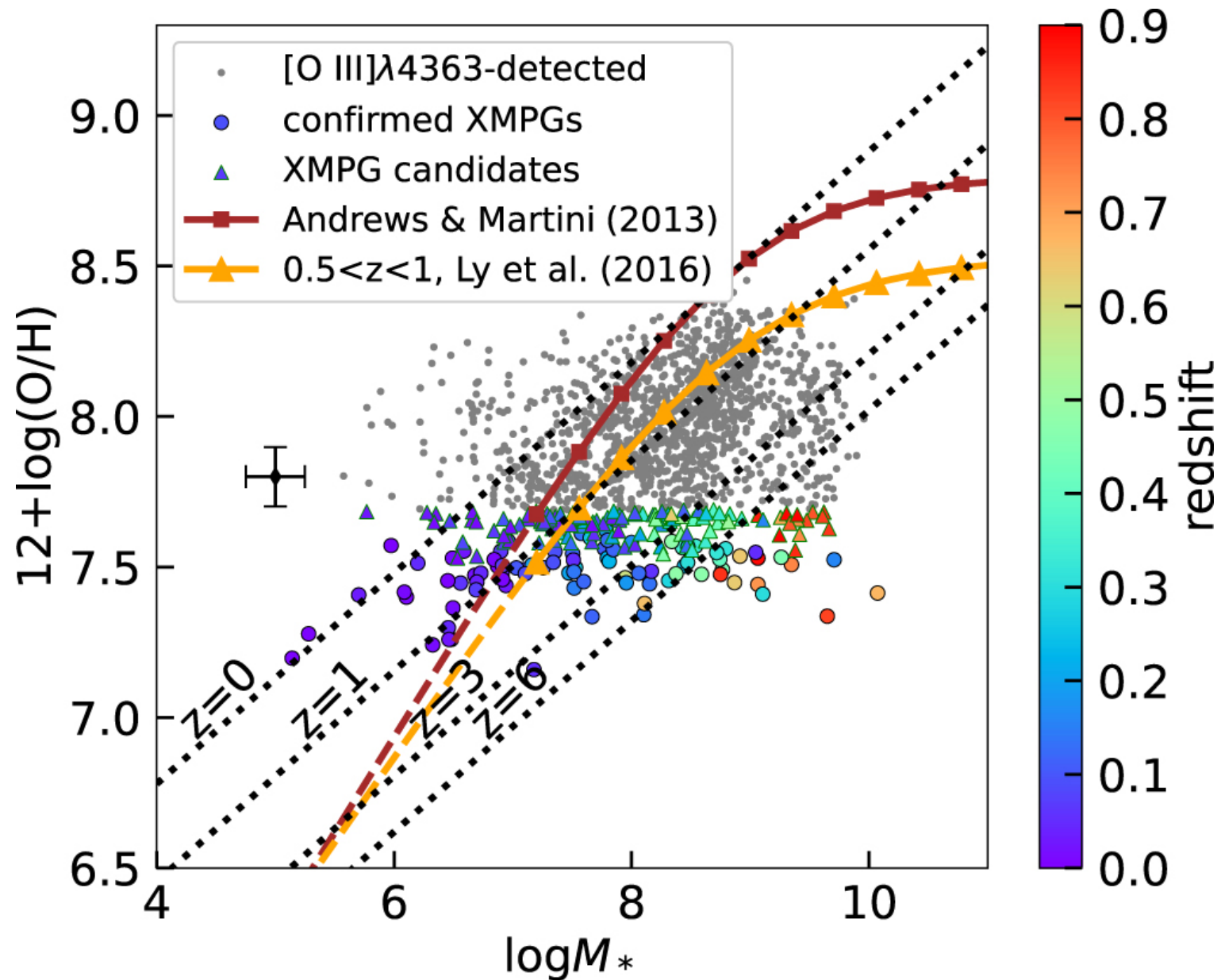
Figure 13. from Hu Zou et al 2024 Astrophys. J. 961 doi:10.3847/1538-4357/ad1409 https://dx.doi.org/10.3847/1538-4357/ad1409 © 2024. The Author(s). Published by the American Astronomical Society.
