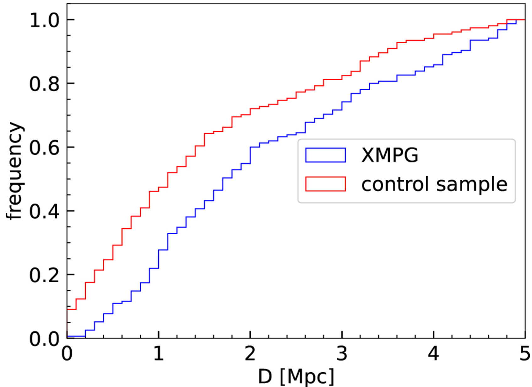
Figure 12. from Hu Zou et al 2024 Astrophys. J. 961 doi:10.3847/1538-4357/ad1409 https://dx.doi.org/10.3847/1538-4357/ad1409 © 2024. The Author(s). Published by the American Astronomical Society.
