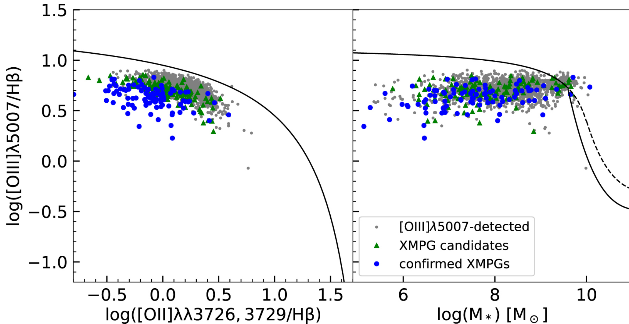
Figure 11. from Hu Zou et al 2024 Astrophys. J. 961 doi:10.3847/1538-4357/ad1409 https://dx.doi.org/10.3847/1538-4357/ad1409 © 2024. The Author(s). Published by the American Astronomical Society.
