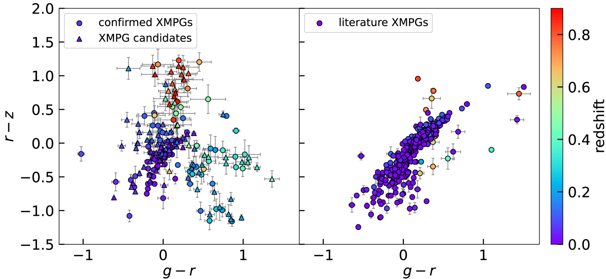
Figure 10. from Hu Zou et al 2024 Astrophys. J. 961 doi:10.3847/1538-4357/ad1409 https://dx.doi.org/10.3847/1538-4357/ad1409 © 2024. The Author(s). Published by the American Astronomical Society.
