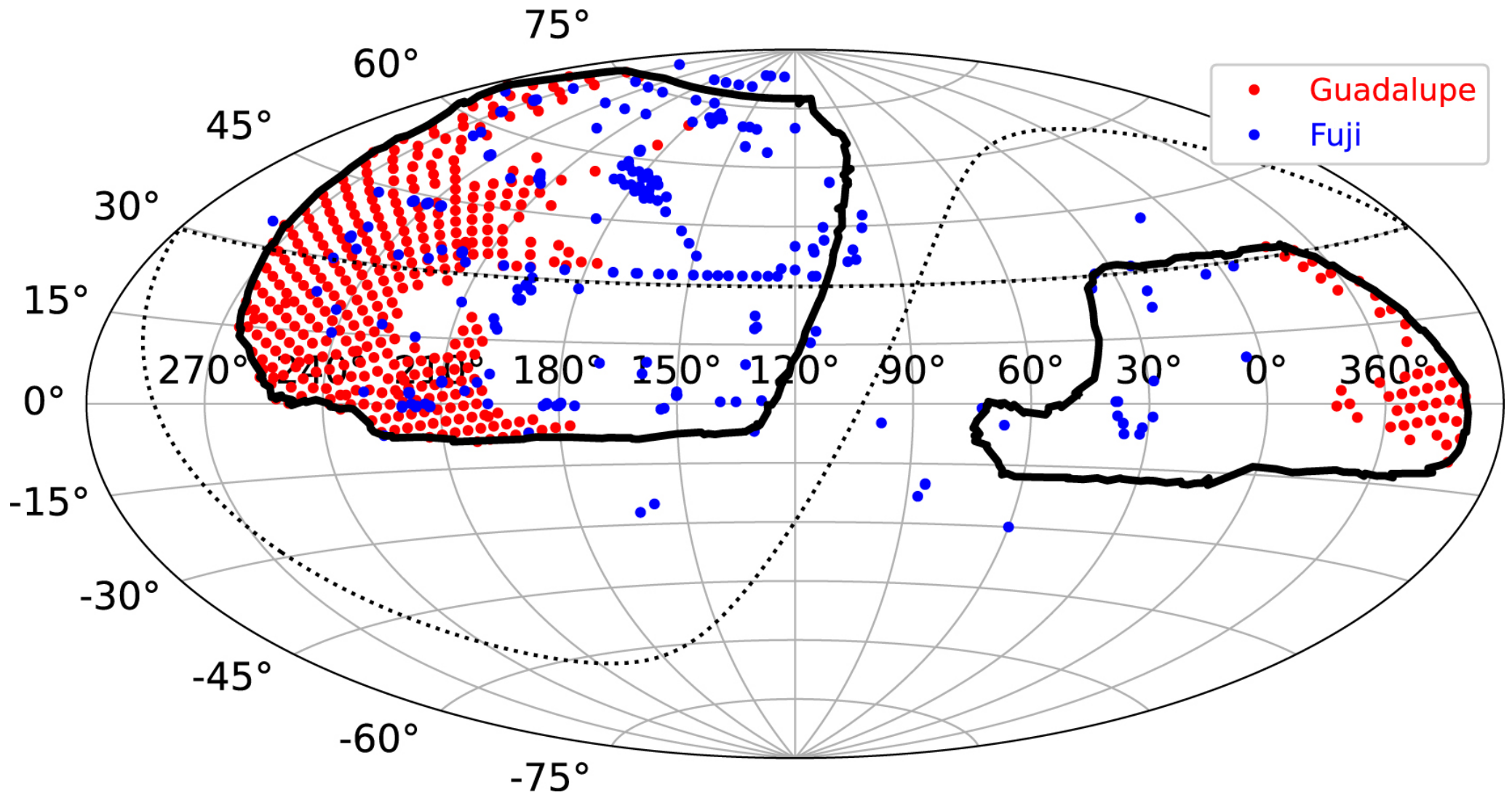
Figure 1. from Hu Zou et al 2024 Astrophys. J. 961 doi:10.3847/1538-4357/ad1409 https://dx.doi.org/10.3847/1538-4357/ad1409 © 2024. The Author(s). Published by the American Astronomical Society.
