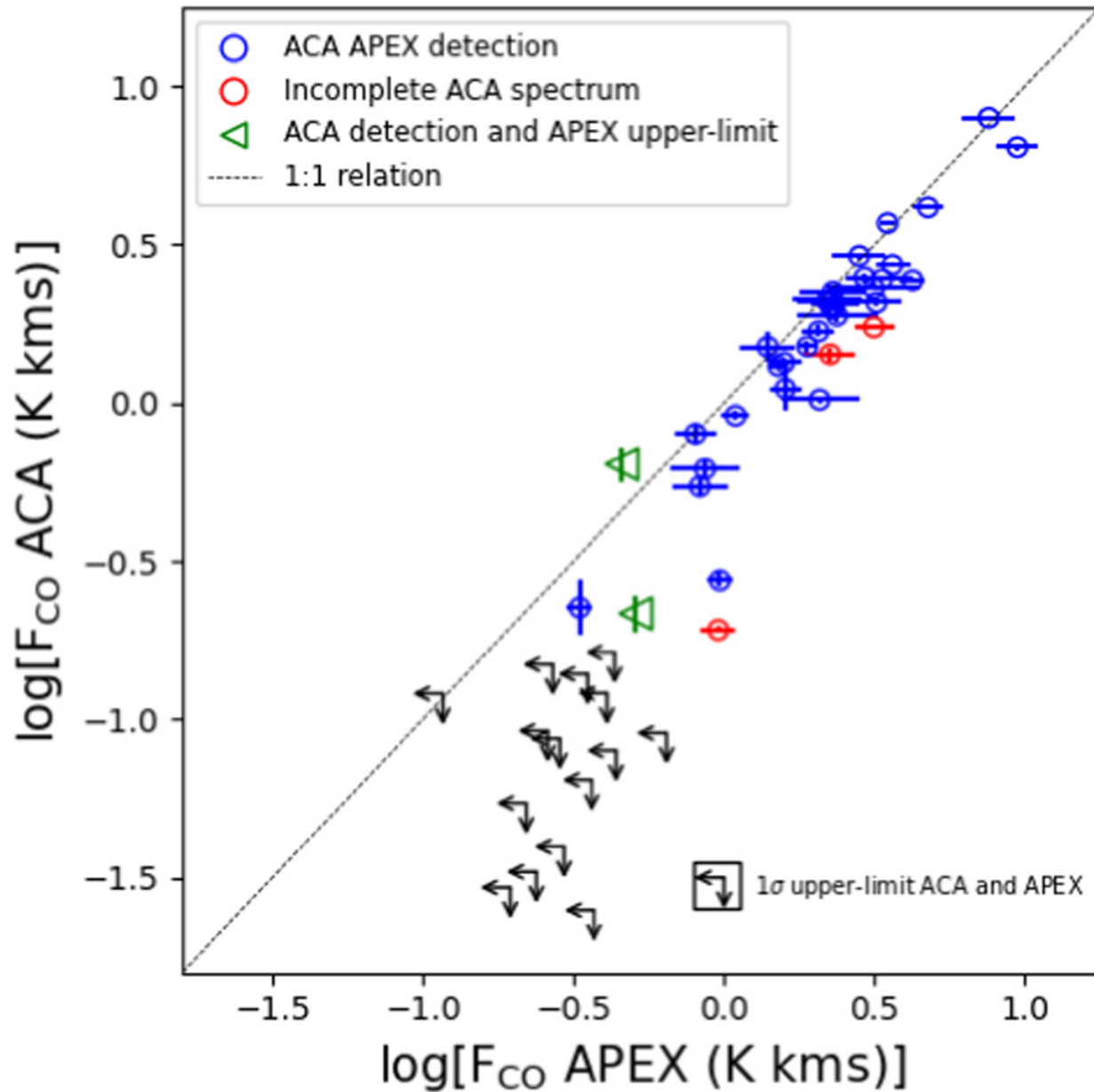
Figure 5. from Vicente Villanueva et al 2024 Astrophys. J. 962 doi:10.3847/1538-4357/ad1387 https://dx.doi.org/10.3847/1538-4357/ad1387 © 2024. The Author(s). Published by the American Astronomical Society.
