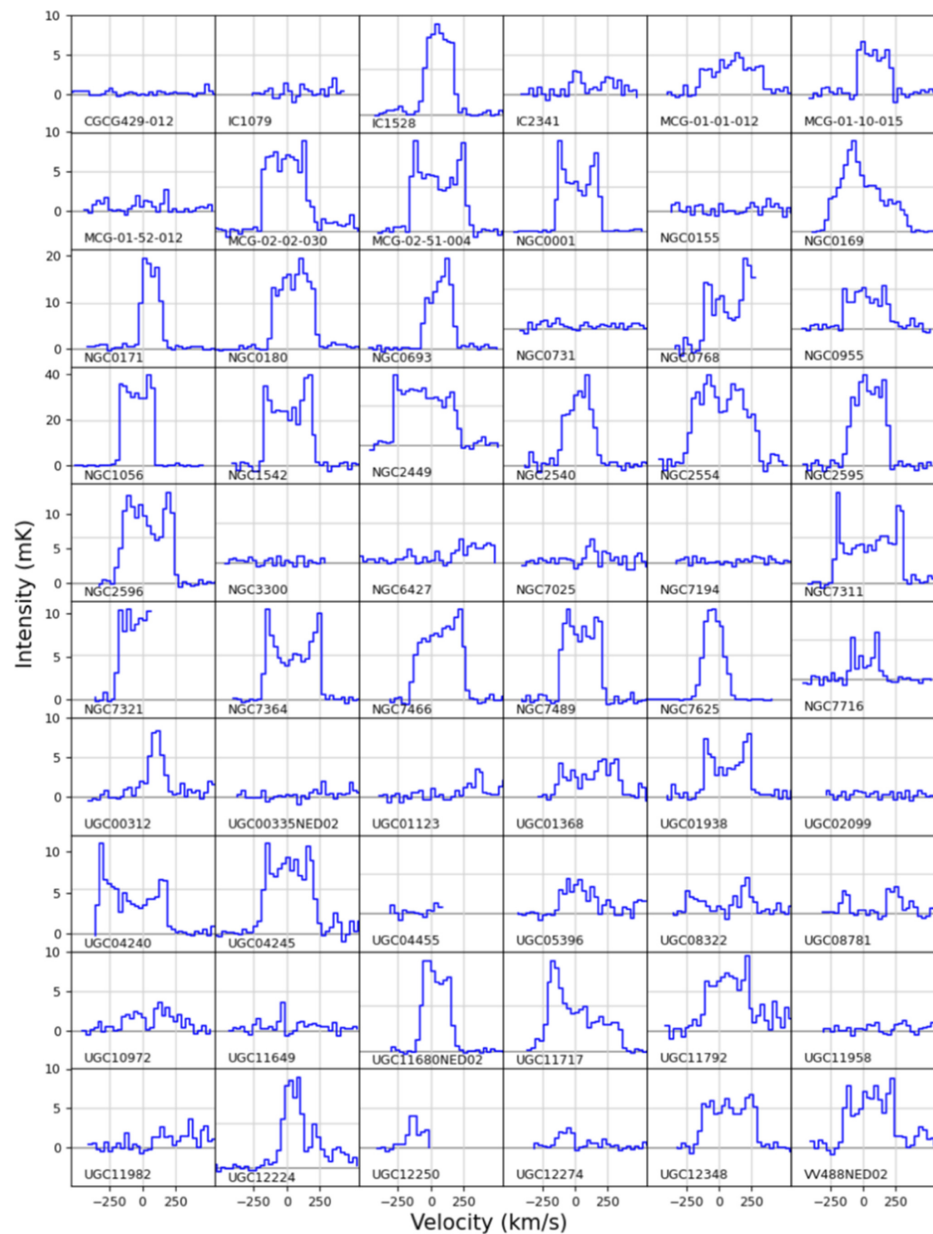
Figure 4. from Vicente Villanueva et al 2024 Astrophys. J. 962 doi:10.3847/1538-4357/ad1387 https://dx.doi.org/10.3847/1538-4357/ad1387 © 2024. The Author(s). Published by the American Astronomical Society.
