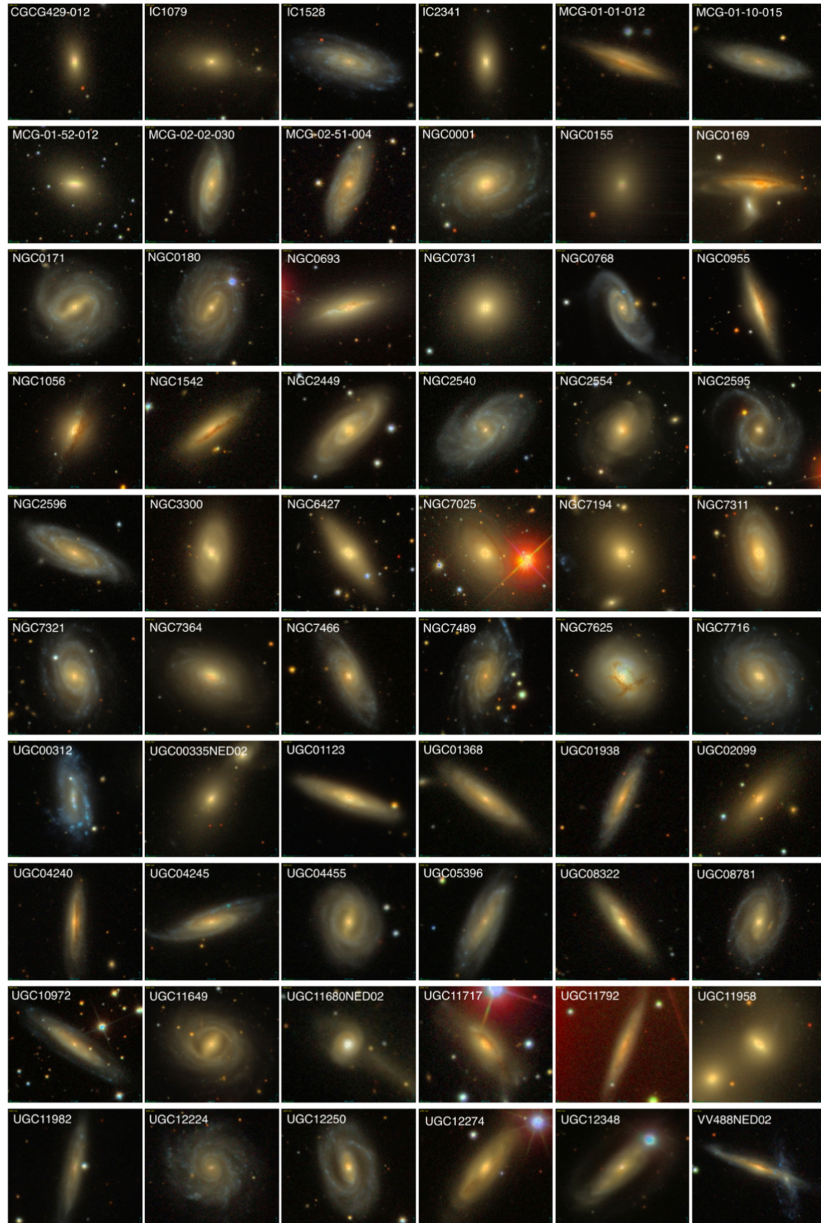
Figure 2. from Vicente Villanueva et al 2024 Astrophys. J. 962 doi:10.3847/1538-4357/ad1387 https://dx.doi.org/10.3847/1538-4357/ad1387 © 2024. The Author(s). Published by the American Astronomical Society.
