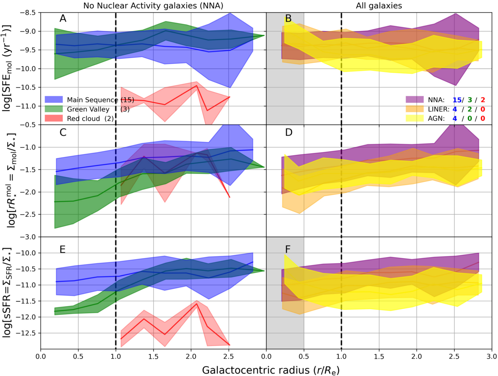
Figure 12. from Vicente Villanueva et al 2024 Astrophys. J. 962 doi:10.3847/1538-4357/ad1387 https://dx.doi.org/10.3847/1538-4357/ad1387 © 2024. The Author(s). Published by the American Astronomical Society.
