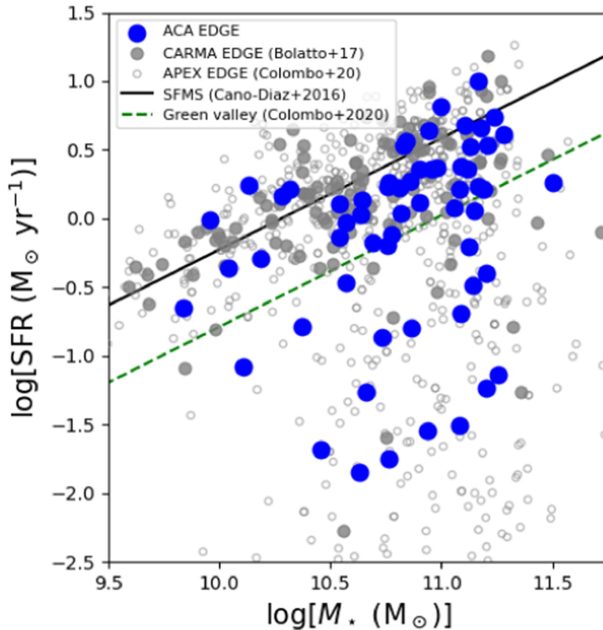
Figure 1. from Vicente Villanueva et al 2024 Astrophys. J. 962 doi:10.3847/1538-4357/ad1387 https://dx.doi.org/10.3847/1538-4357/ad1387 © 2024. The Author(s). Published by the American Astronomical Society.
