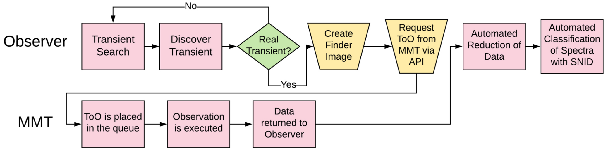
Figure 12. from Manisha Shrestha et al 2024 Astrophys. J. 961 doi:10.3847/1538-4357/ad11e1 https://dx.doi.org/10.3847/1538-4357/ad11e1 © 2024. The Author(s). Published by the American Astronomical Society.
